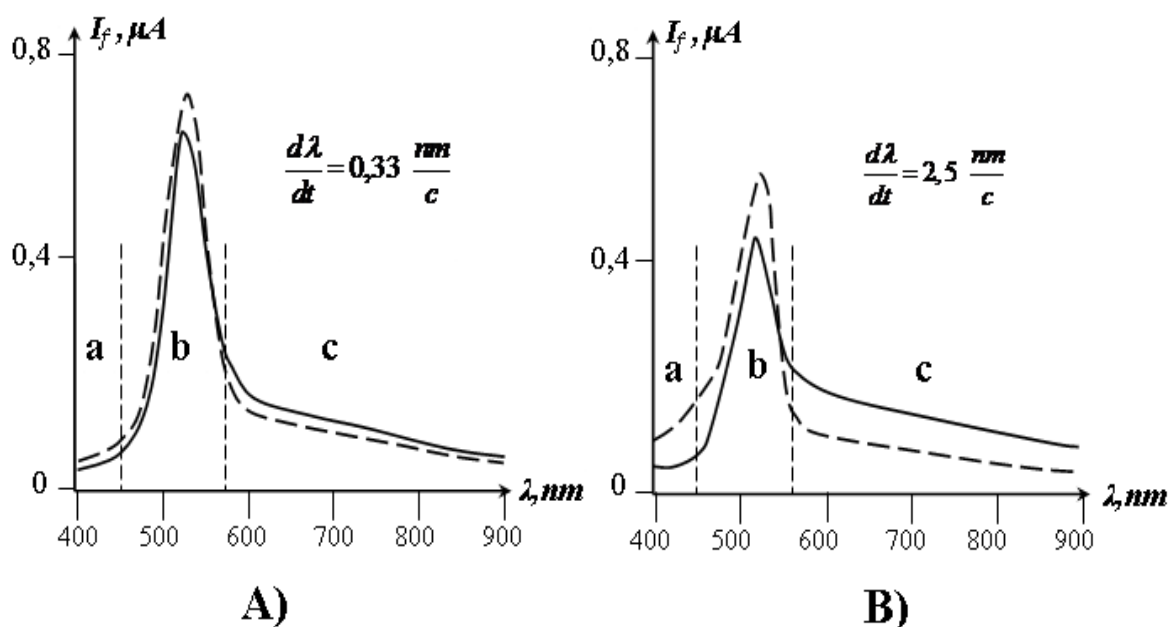
Fig. 6.1. Typical curves of the spectral distribution of the photocurrent of the studied samples when the wavelength changes from small to large values (solid line) and from large to small (dotted line). The speed of change in the wavelength of light: A) – 0.33 nm/s and B) – 2.5 nm/s. в рисунке исправить с на s.
