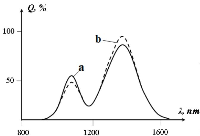
Fig. 7.3. Influence of temperature on the spectral distribution of the quenching coefficient. a ) - measurements were made at 24 °C; b ) - the temperature was 50 °C..
