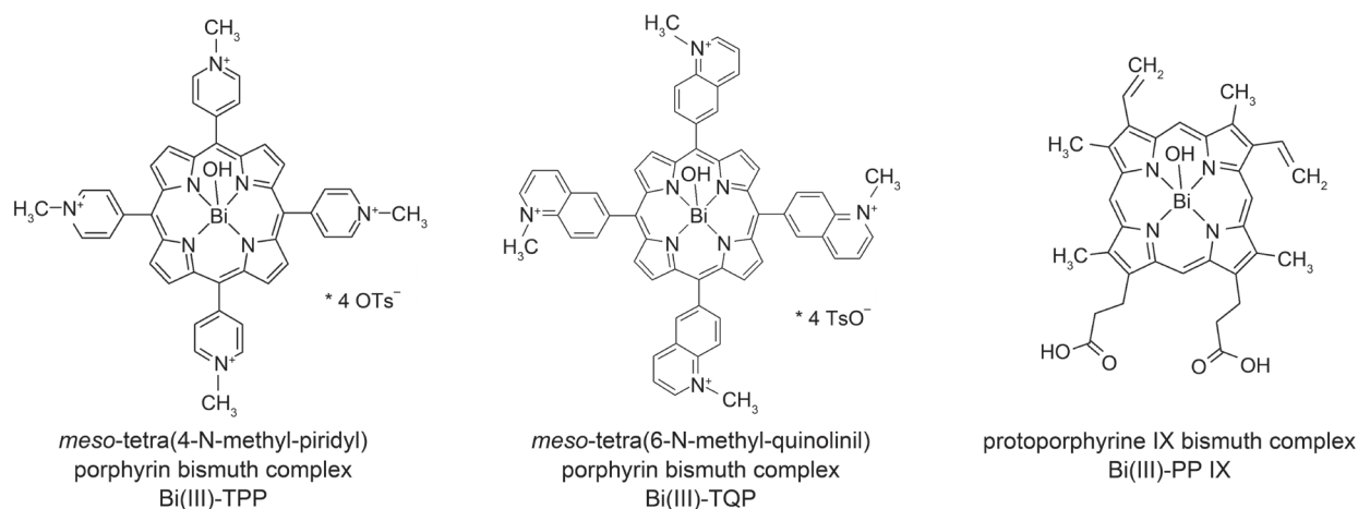
Fig. 1. Porphyrins bismuth complexes, used in the study
