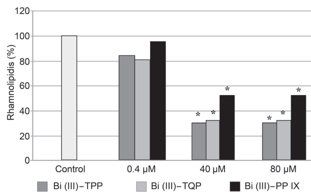
Fig. 2. Rhamnolipids biosynthesis by P. aeruginosa PA01 after pre-incubation with porphyrins bismuth complexes
