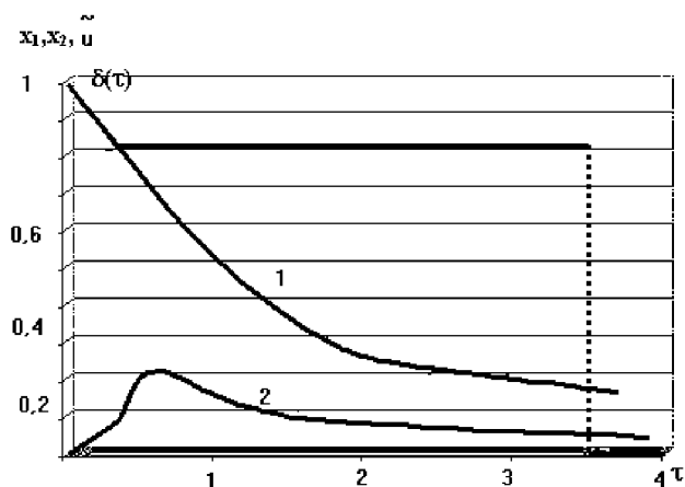
Fig. 4. Results of modelling Ga separation process from Ga-X mixture by the photo-ionization method ( \delta —dashed — laser pulse optimal form; curves x_1 , x_2 are corresponding to populations of the ground and excited states)
