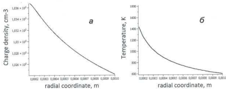
Fig. 2. Calculated dependence of the charge density of the radial coordinate (a) and calculated dependence of the air temperature around the copper particle (b).
