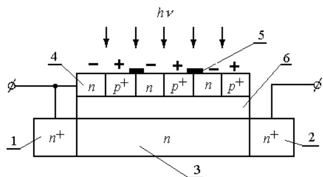
Fig. 1. Structure of the MIS-phototransistor. 1 — source, 2 — drain, 3 — channel of conductance, 4 — gate, 5 — shunting bridge, 6 — dielectric.
