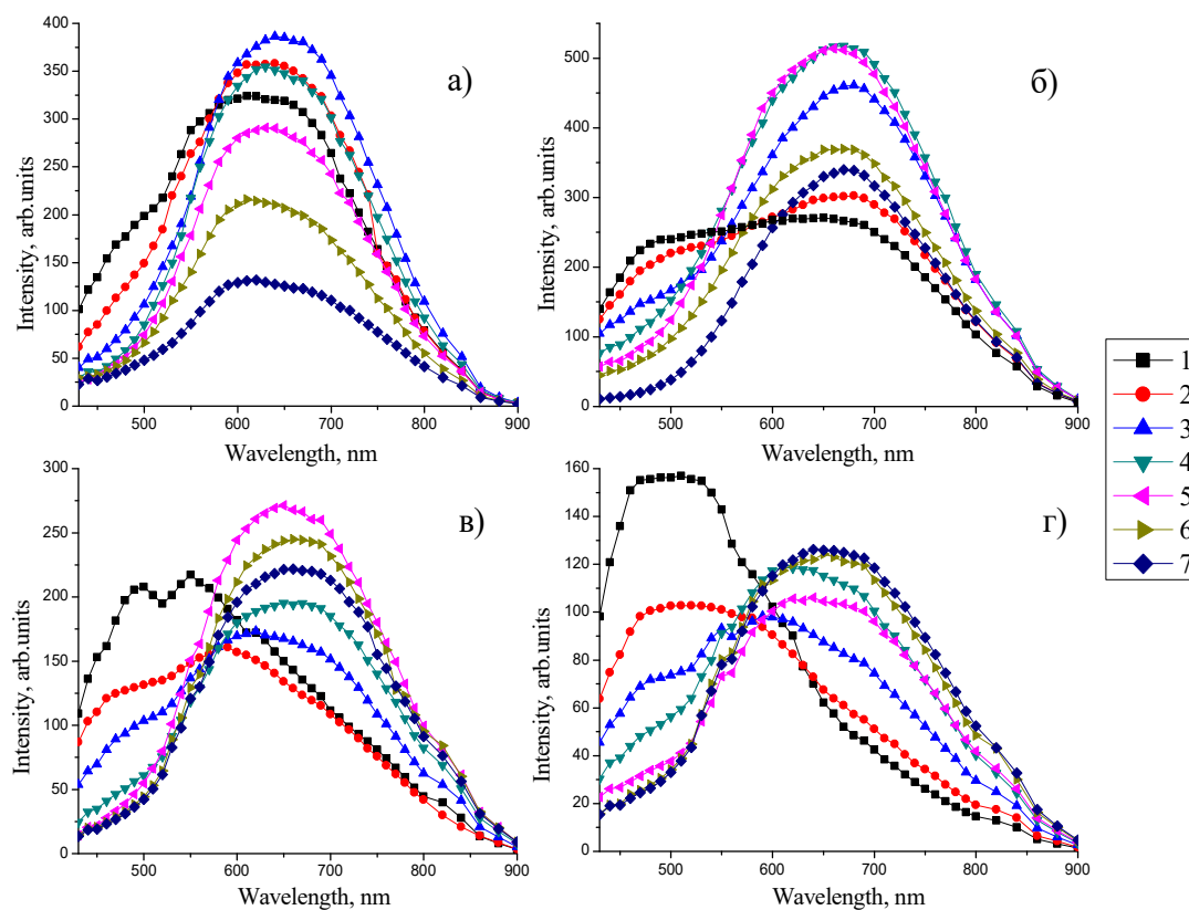
Fig. 6 – Luminescence spectra of CdS QDs obtained at the molar ratio of the initial components \text{CdNO}_3 / \text{Na}_2\text{S} : 1/4 (a); 1/2 (b); 1/1 (c); 2/1 (g).
