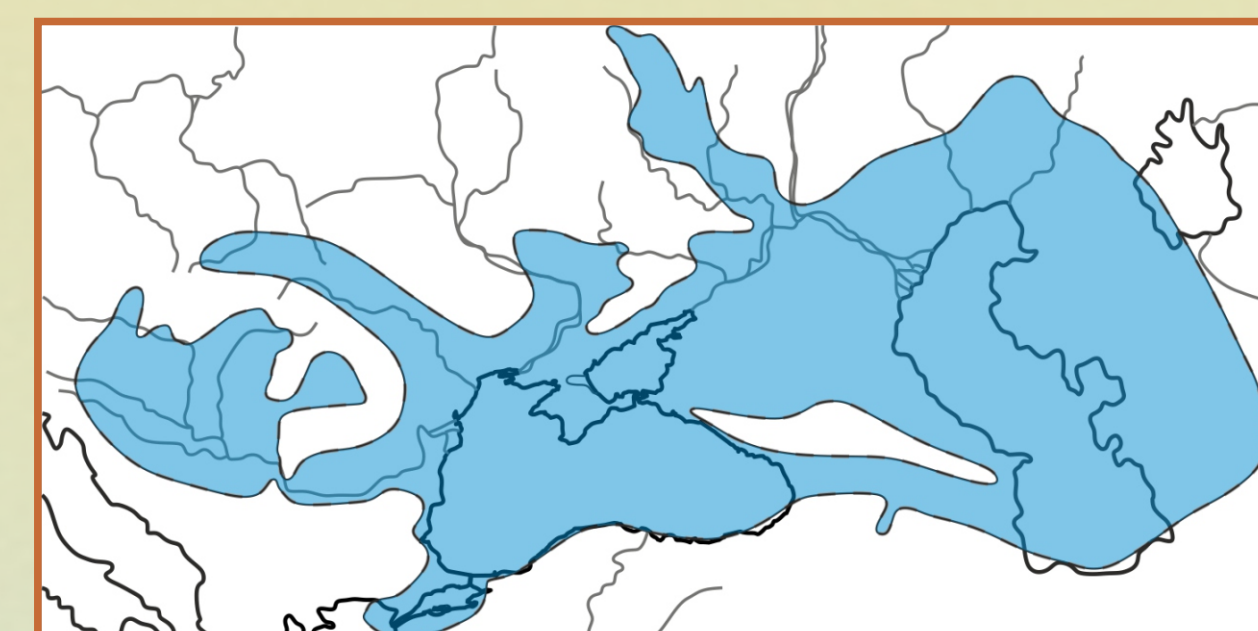
Figure 2. Maximal configuration of the Sarmatian Sea-Lake shorelines according to the results of geologic research [6].
