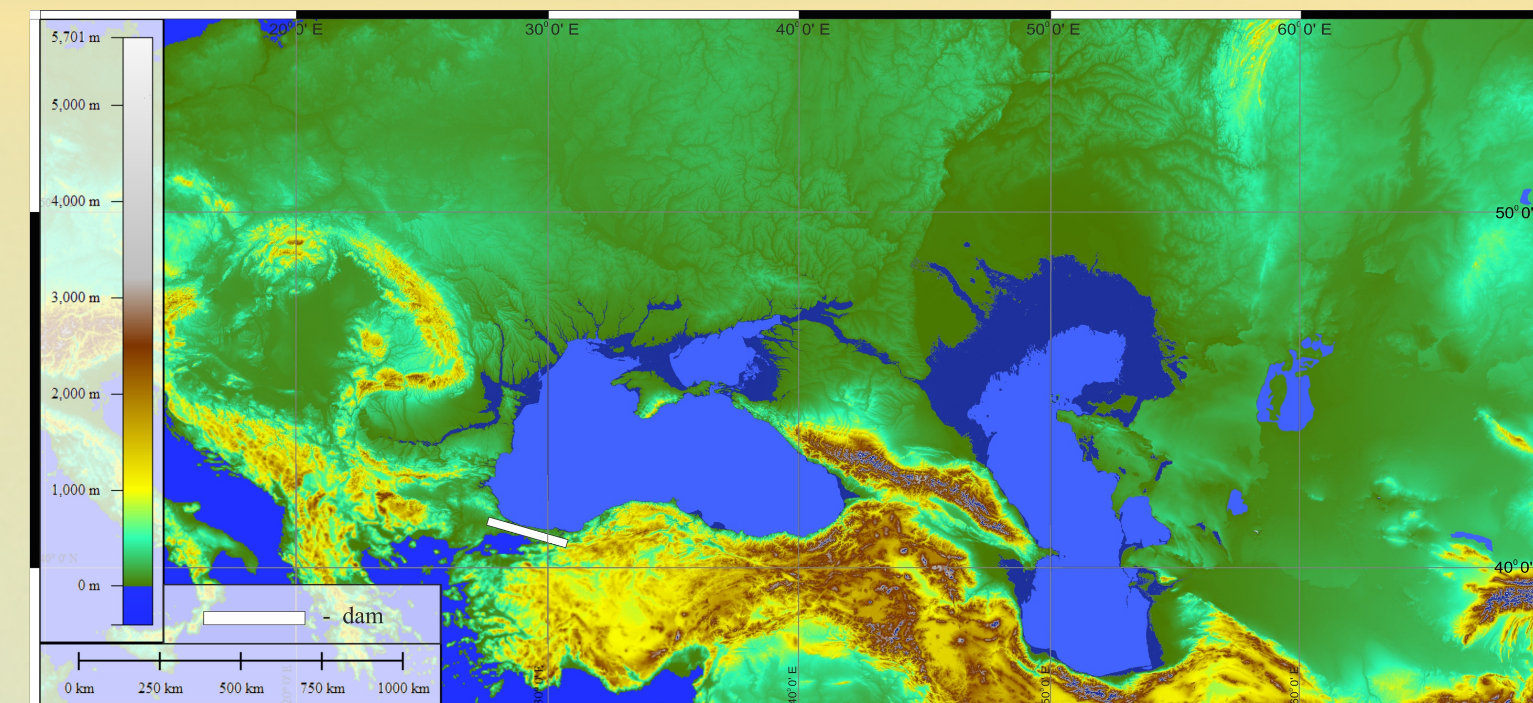
Figure 5. The Black Sea-Caspian Sea region under present climatic conditions in which communication with the Marmara Sea is blocked. Possible hydro-isostasy changes in topography have not been considered.
