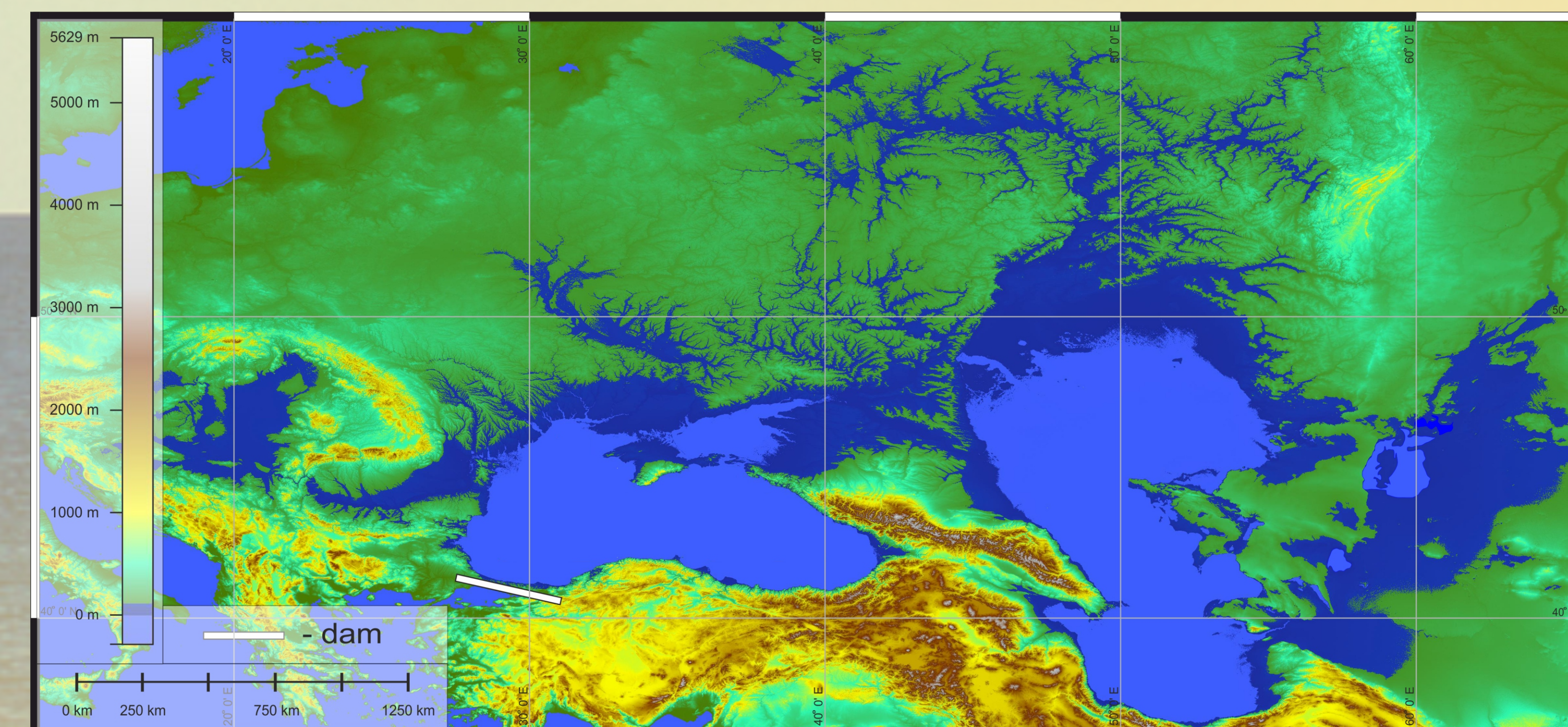
Figure 6. Sea-lake, which would have formed during the period of intensive glacial melting and blockage of the connection with the Sea of Marmara. The sea-lake level would rise 116 m. The shape of the coastline would resemble the coastline of the Sarmatian Sea-Lake (see Figure 2).
