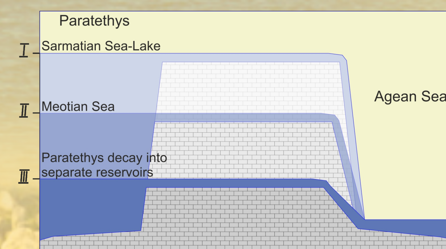
Figure 7. Scheme of the Paratethys Sea-Lake deepening under conditions of bridge erosion. In this scheme, three positions of the canyon bottom are shown crossing the mountain range between the Black and the Aegean seas. The erosion base level is a regressive level of the Aegean Sea.
