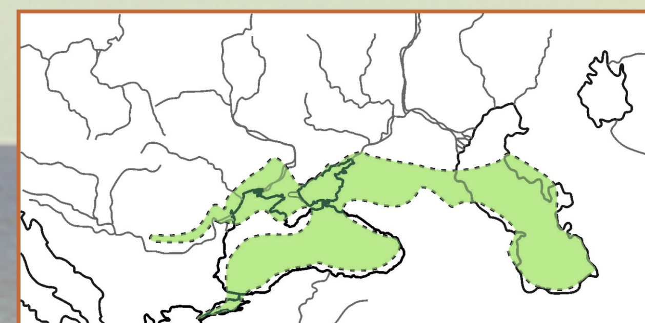
Figure 3. Meotian Sea according to the results of geologic research [6].
