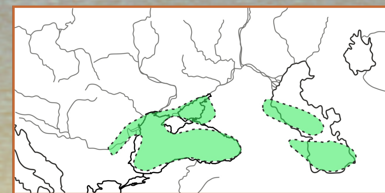
Figure 4. Middle Pliocene, the stage of decay into separate reservoirs [9, 7].
