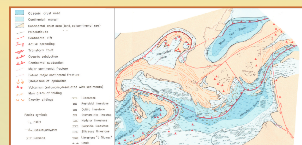
Figure 1. Paleogeographic map of the Black Sea-Mediterranean Sea region in the Tortonian [1]. A mountain massif separates the Black and the Mediterranean seas.
