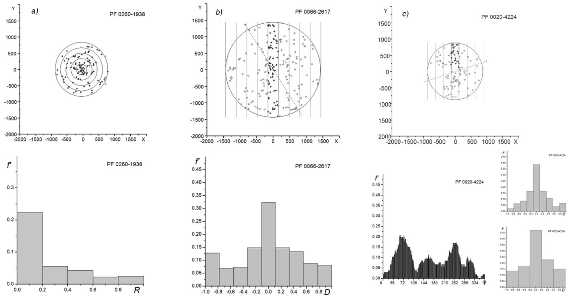
Figure 3: The examples of the analysis of cluster' features: a ) 23% of galaxies located in 1/25 part of the cluster area – C-type; b ) no central concentration and 33% of galaxies located in middle stripe from 9 ones – OL9 cluster; c ) X-type peculiarity, the distribution of densities in the “lighthouse beam” histogram has 4 maxima and corresponded L9 and L5 histograms are shown this type clearly. The map for this cluster is shown in Fig.2
