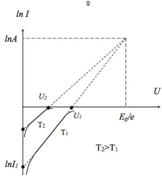
Fig. 4. VAC lines at different temperatures.
