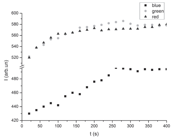
Figure 7. The reflection after ammonia exposure of samples No 1; ammonia concentration 20 ppm.
