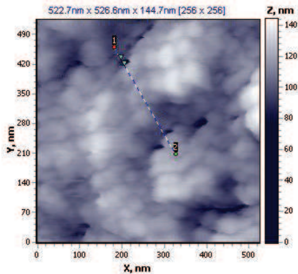
Figure 3. AFM image of Si(100) with a resistivity of 4 Ohm cm after 10 minutes etching in solution— H_2O_2/H_2O/HF = 25/80/40 . Ag particles were deposited before etching in solution 0.23M HF and 5 \times 10^{-5}M AgNO_3 within 15min
