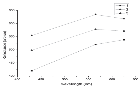
Figure 6. Dependences of maximal magnitudes of reflectance for samples No 2 under nitrogen (curve 1) and different concentrations of ammonia (curve 2 – 20 ppm, 3 – 60 ppm).
