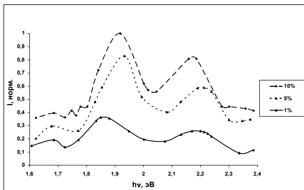
Fig. 3. The photoluminescence spectrum of \text{SnO}_2 films with different concentrations of the precursor (0.05% PVA) at room temperature.
