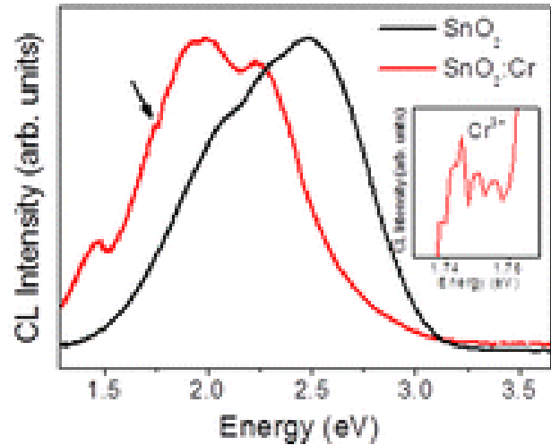
Fig 1. The normalized emission spectra \text{SnO}_2 and \text{SnO}_2\text{:Cr} . [25]
