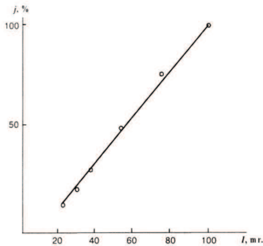
FIG. 3. Dependence of video-signal amplitude on the dose of incident X-ray radiation
