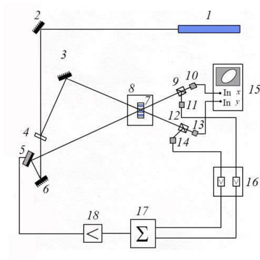
Fig.3.5. Schematic diagram of the installation: 1 – LGN-215 laser; 2, 3, 6 – mirrors; 4 – light divider; 5 – mirror mounted on a piezoelectric crystal; 7 – sample; 8 – oven-thermostat mounted on a rotary table; 9, 12 – light-separating cube; 10, 11, 13, 14 – photodiodes; 15 – oscilloscope; 16 – differential amplifier; 17 – integrator; 18 – high-voltage amplifier.
