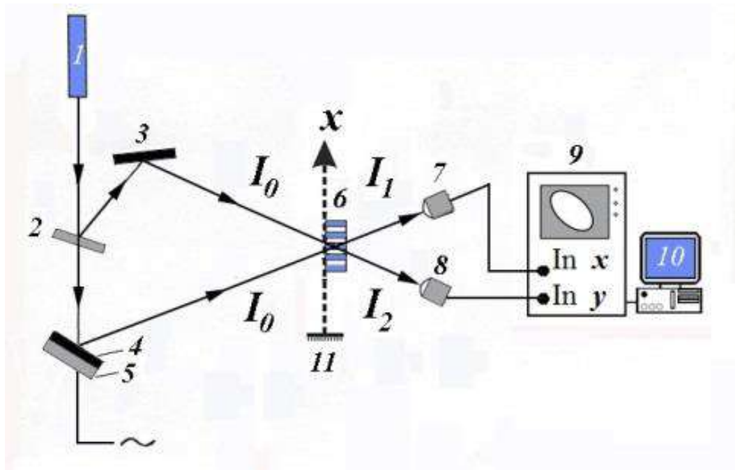
Fig.3.6. Schematic diagram of the installation for determining the amplitude and phase modulations when recording the amplitude-phase lattice.
