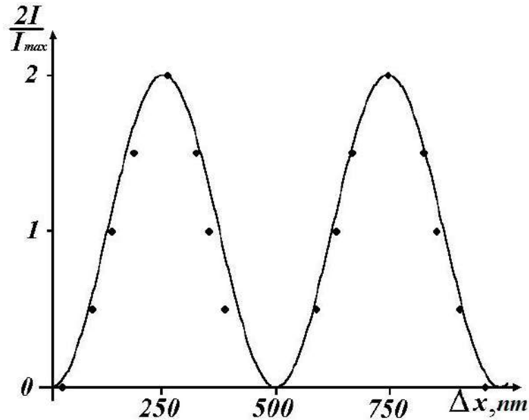
Fig.4.9. Dependence of the magnitude of the output signal I from the photodiode 8 (Fig.4.7) on the offset \Delta x of the object.
