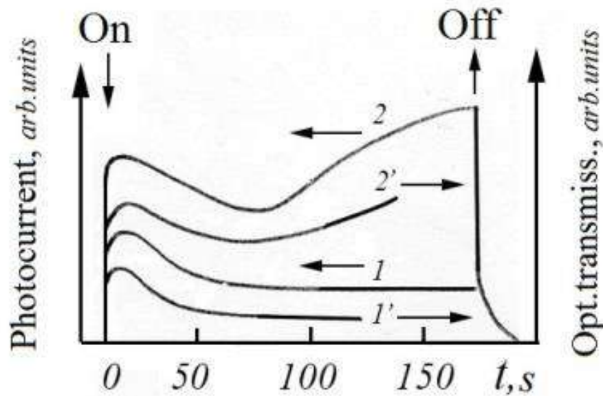
Fig.2.20. Kinetics of photocurrent (curves 1, 2) and optical transmission (curves 1', 2') when the sample As_2S_3 is excited by rectangular pulses of He-Ne laser light with a power of 0,1 \text{ W/cm}^2 : 1,1'– 35^\circ\text{C} ; 2, 2'– 150^\circ\text{C} .
