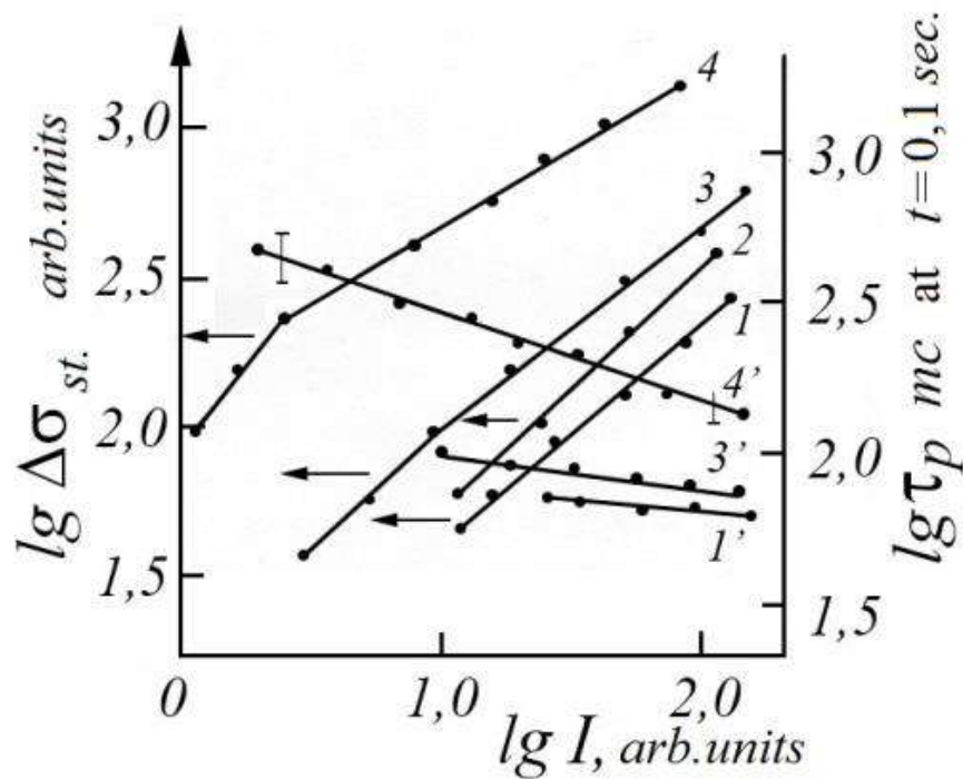
Fig.2.8. Lux-ampere characteristics (1–4) depending on \tau_p (1'–4'), determined by formula (2.19), for the moment of time t=0,1 sec from the light intensity of the He-Ne laser for As_2S_3 at different temperatures ( \omega=290 Hz).
