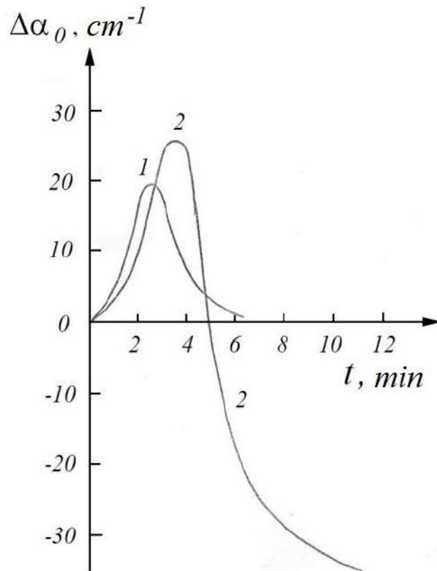
Fig.3.14. Kinetics of change of amplitude of modulation of absorption coefficient ( \Delta\alpha'_0 ) in the process of recording lattice in crystals: 1 – KBr ; 2 – KCl .
