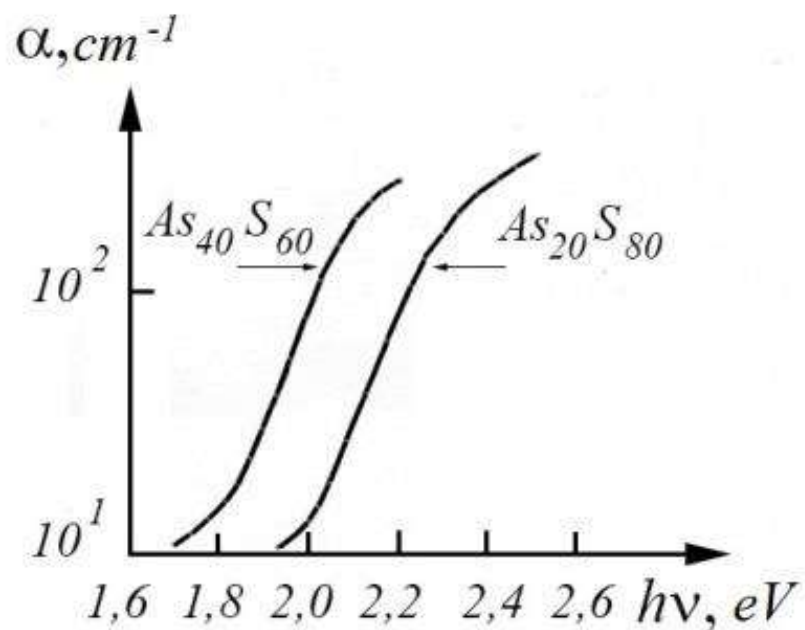
Fig.2.5. Spectral dependence of the absorption coefficient \alpha(h\nu) for system samples As-S with different sulfur content.
