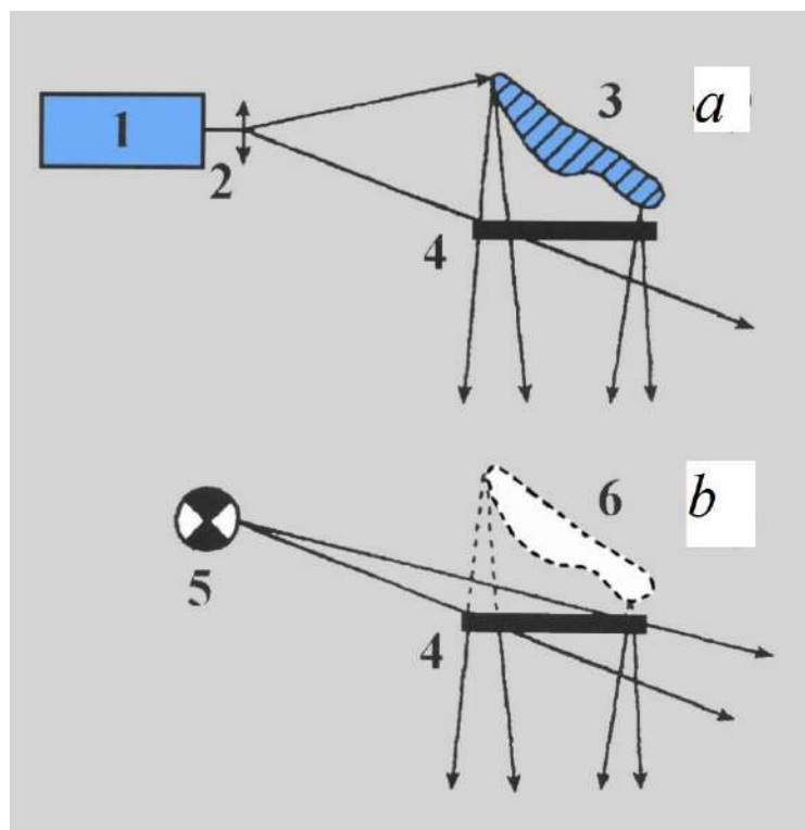
Fig.3.4. The scheme of recording three-dimensional transmitting holograms in converging beams: (a) – recording scheme, (b) – recovery scheme.
