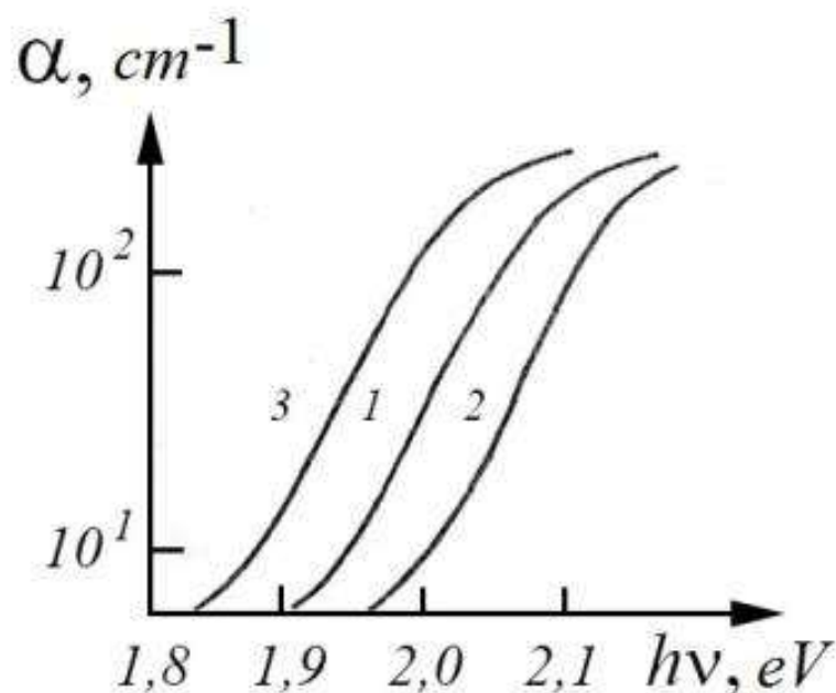
Fig.2.17. The self-absorption edge As_2S_3 , measured at 55^\circ C , after annealing at 180^\circ C (curve 1) and exposed at 160^\circ C (He-Ne laser) and 20^\circ C (Xe -lamp) (curves 2, 3, respectively).
