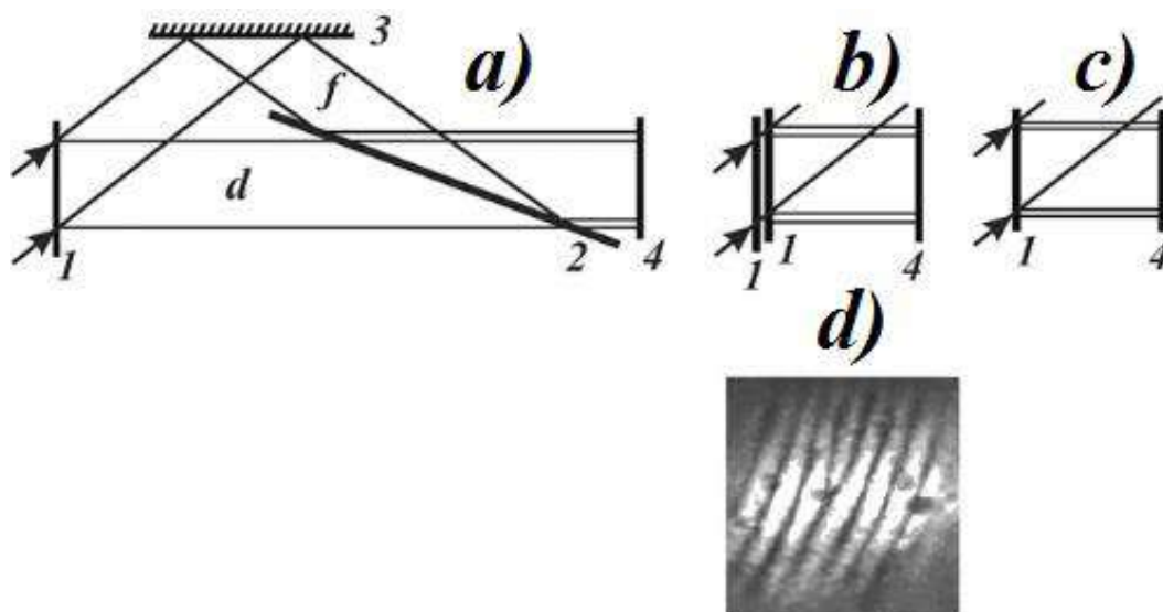
Fig.4.24. Possible options for restore of beams from SD and beams-analyzers: 1 – hologram (HOE), 2 – translucent dividers, 3 – mirror, 4 – screen.
