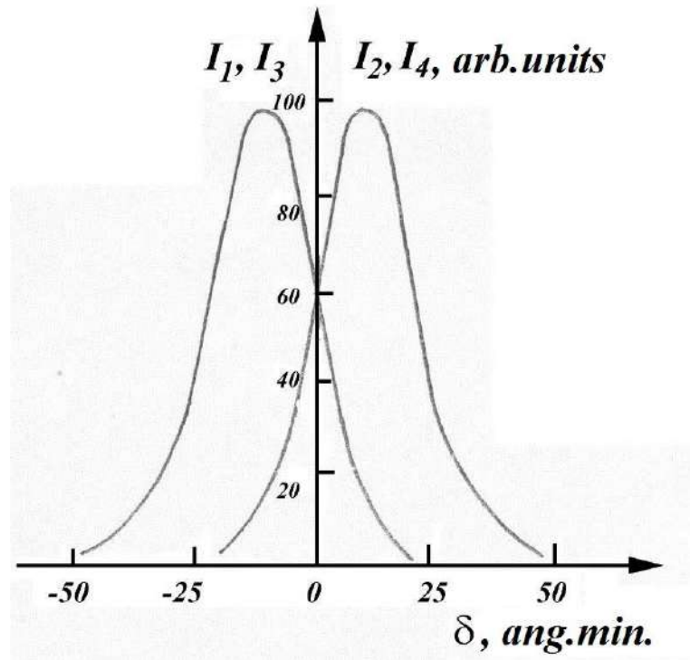
Fig.4.19. Angular dependence of the intensity of diffracted beams on the first I_1 , second I_2 , third I_3 and fourth I_4 sublattices: I_1, I_2 – when rotating the HOE relative to the axis Oy ; I_3, I_4 – relative to the axis Ox .
