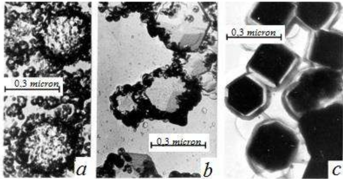
Fig.1.8. Photomicrographs illustrating the results of different crystallization options AgBr on the surface of CaF_2 microcrystals under the conditions: a ) low pBr (from 1,3 to 2,0), b ) medium pBr (from 2,0 to 4,0), c ) high pBr up to 7,0) (solubility AgBr ( PS = [Ag^+] \cdot [Br^-] = 5,3 \cdot 10^{-13} )).
