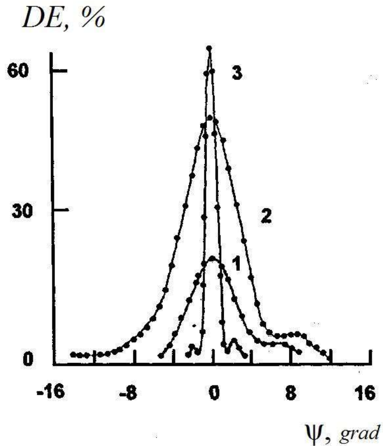
Fig.3.3. Angular selectivity of transmitted elementary holograms recorded on: 1 – PFG-03; 2 – PFG-04; 3 – emulsion with heterophase microsystems "core \text{CaF}_2 –shell \text{AgBr(I)} ".
