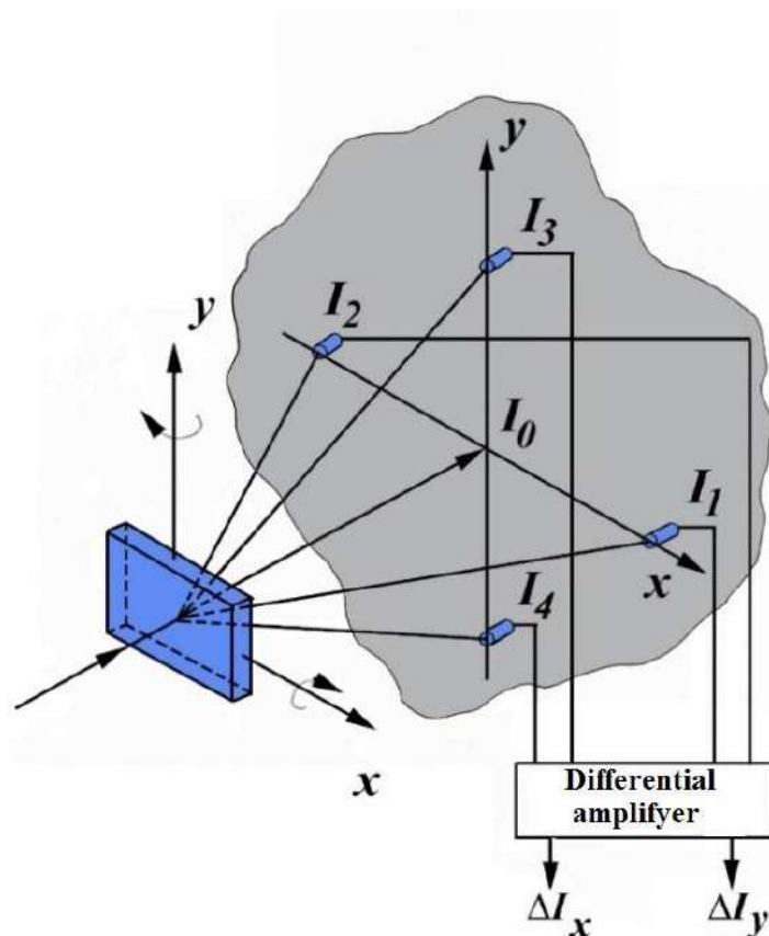
Fig.4.18. Diffraction of light on HOE – medium, in the volume of which four three-dimensional diffraction gratings are recorded: I_0 – beam of passing light; I_1, I_2, I_3 and I_4 – light beams diffracted on 1, 2, 3 and 4 sublattices, respectively.
