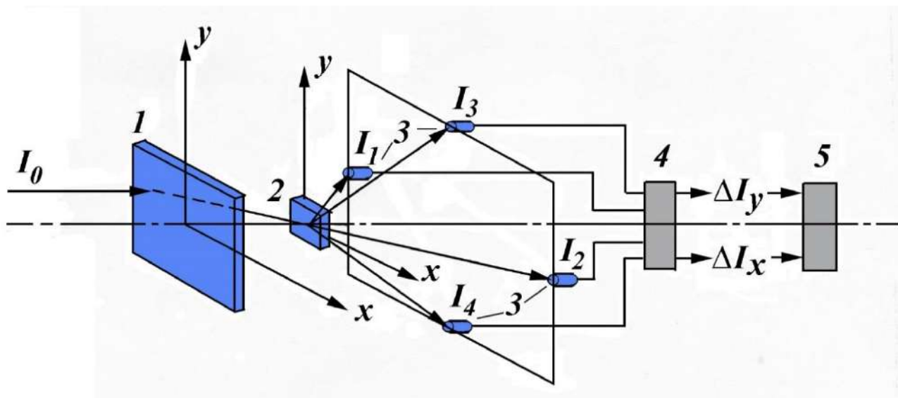
Fig.4.21. Schematic diagram of a two-coordinate sensor of the position of the laser beam based on HOE: 1 – holographic lens; 2 – HOE, consisting of 4 sublattices; 3 – photodetector; 4 – differential amplifier; 5 – indicator device.
