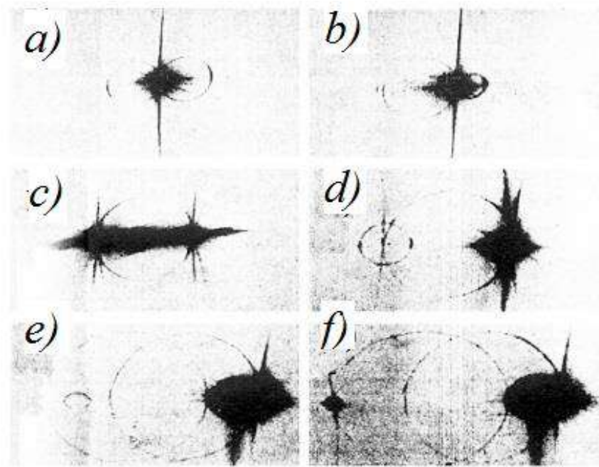
Fig.3.21. The reducing ray lies in the plane of the recording rays. The angle \varphi of incidence varies from 0 to 2\theta .
