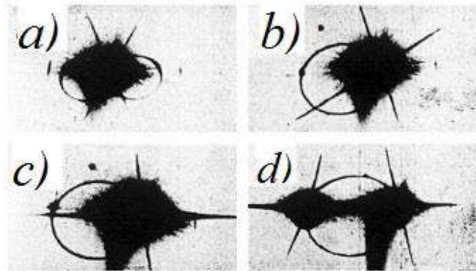
Fig.3.23. The reducing ray is derived from the plane of the recording rays. The angle \varphi of incidence in the plane of the recording rays varies from 0 to Bragg ( \theta ):
