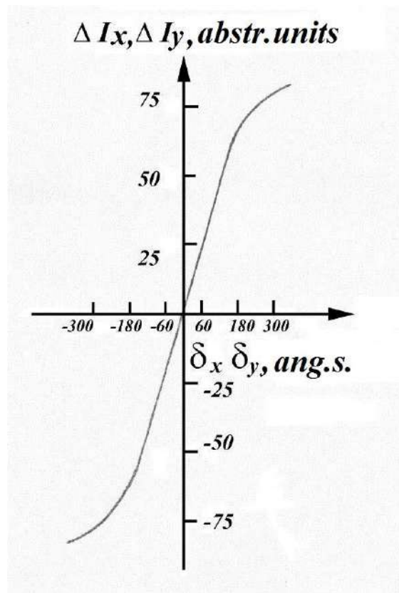
Fig.4.20. Dependence of the output values of the differential amplifier signal \Delta I_y and \Delta I_x from the angle of rotation of the HOE.
