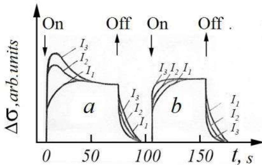
Fig.2.19. Kinetics of photoresponsiveness at primary (a) and repeated (b) illumination, change at different intensities of exciting light ( I_1 < I_2 < I_3 ) in As_2S_3 .
