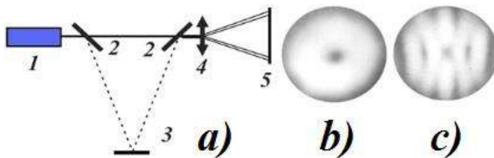
Fig.4.22. a) SD scheme in laser radiation that generates Lagerr-Gaussian mode (1 – LG-75 laser, 2 – translucent dividers, 3 – mirror, 4 – lens, 5 – screen);
