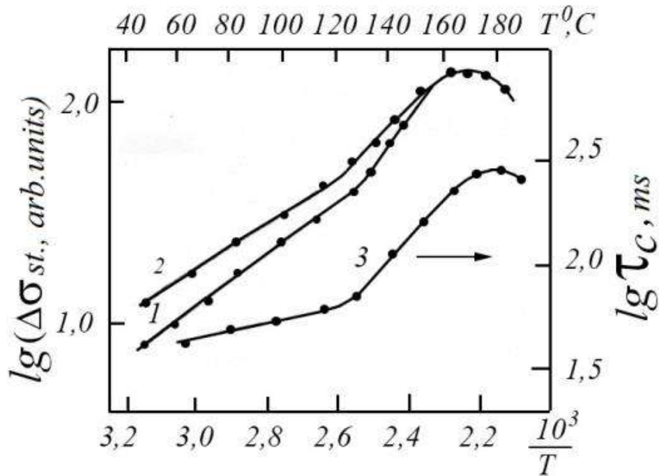
Fig.2.11. Temperature dependence \Delta\sigma_{st} (curves 1, 2) and \tau_c , determined by formula (2.20) (curve 3): 1, 3 – sample \text{As}_2\text{S}_3 which before each measurement is annealed at T \approx 180^\circ\text{C} for 15 minutes; 2 – sample \text{As}_2\text{S}_3 illuminated by He-Ne laser light at T=140^\circ\text{C} for 15 minutes ( \omega = 290 \text{ Hz} ).
