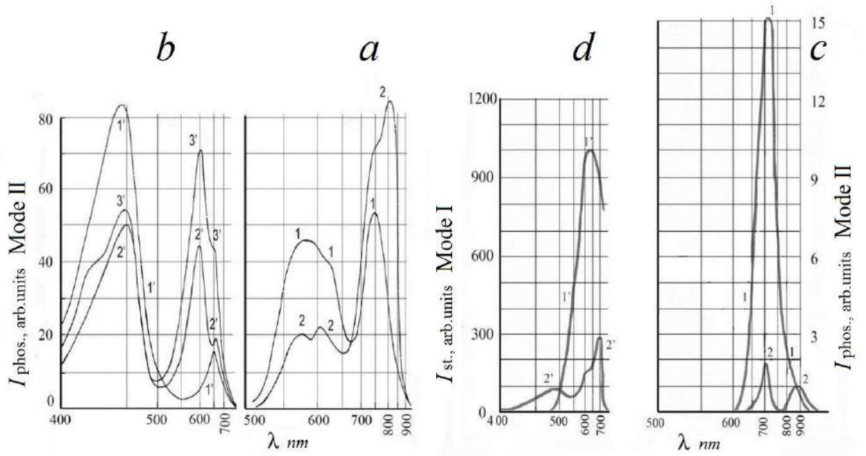
Fig.1.16. a) Luminescence spectra at T=77K emulsion type G, measured in phosphorescent mode when excited by light wavelength \lambda (nm): 1–430; 2–690.
