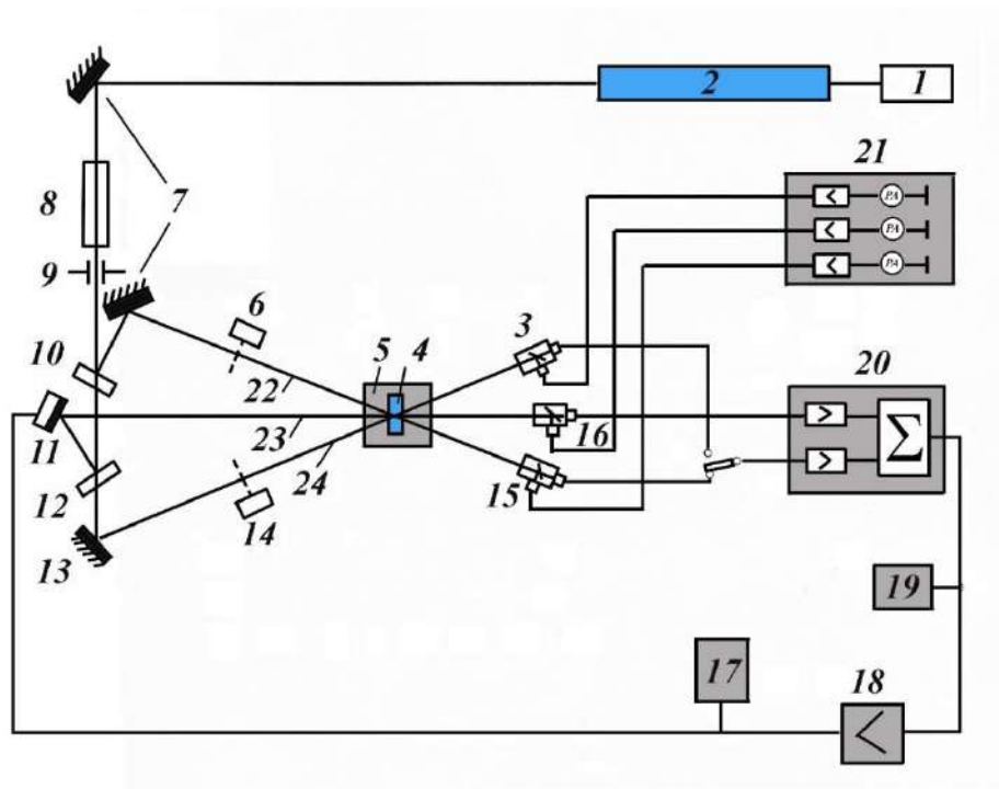
Fig.4.16. Schematic diagram of a device for recording a three-dimensional combined grating: 1 – laser power supply; 2 – laser; 3, 15, 16 – photodiodes; 4 – three-dimensional light-sensitive environment; 5 – oven-thermostat, which is installed on the turntable; 6, 14 – bolts; 7, 13 – mirrors; 8 – beam expander; 9 – diaphragm; 10, 12 – light divider; 11 – mirror mounted on piezoceramics; 17, 19 – oscilloscopes; 18, 20, 21 – electronic blocks of the system of stabilization and determination of holographic characteristics of sublattices; 22, 23, 24 – recording beams.
