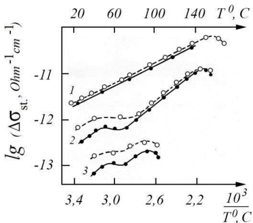
Fig.2.12. Temperature dependence of static (solid curve) and dynamic (dashed curve) photoconductivity ( \omega=500 Hz): 1 – As_2S_3 , 2 – As_{25}S_{75} , 3 – As_{20}S_{80} .
