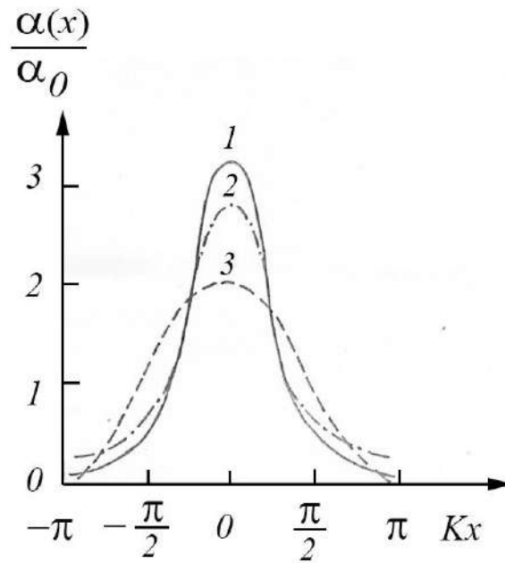
Fig.3.16. Profile of the lattice normalized by the average absorption:
