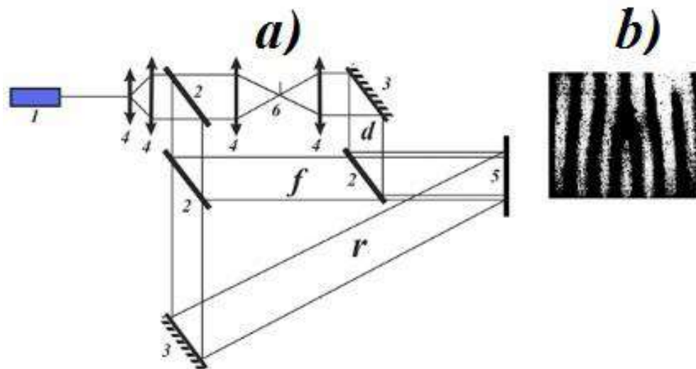
Fig.4.23. a ) Scheme of conversion of a beam with a flat front into a beam with SD and its subsequent registration (1 – laser, 2 – translucent dividers, 3 – mirror, 4 – lenses, 5 – screen or holographic plate, 6 – cover glass, letters are marked: d – beam with dislocation, f – beam-analyzer with a flat front, r – reference beam for hologram recording);
