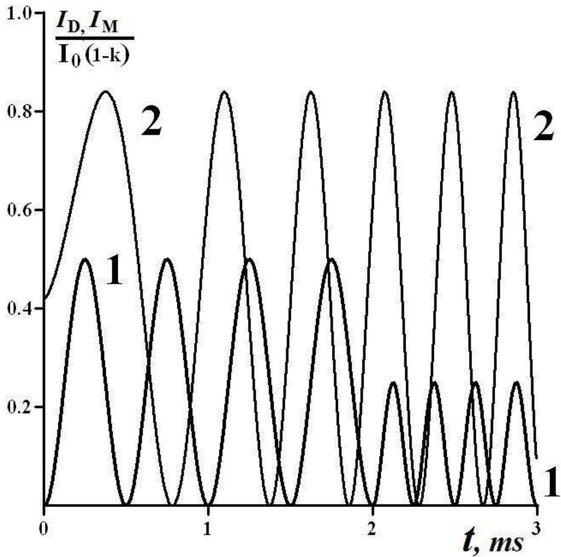
Fig.4.2. Modulating light flux: 1– I_D according to the single-beam scheme, 2– I_M according to the two-beam scheme.
