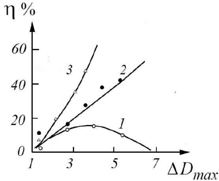
Fig.3.18. Dependence of DE on the amplitude of optical density \Delta D_{max} modulation. Experimental values of DE for \Delta D(\omega) in the case of bands: ○ – symmetric; ● – asymmetric; Δ – \Delta D(\omega_c) \approx 0 .
