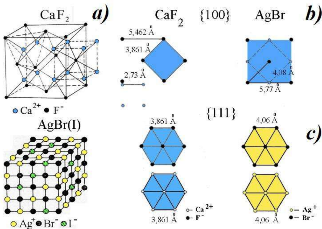
Fig.1.2. a) Elemental \text{CaF}_2 cell and statistical picture of solid solution \text{AgI} in \text{AgBr} ; b) Location of ions in fluorite and silver bromide on planes \{100\} ; c) Location of ions in fluorite and silver bromide on the planes \{111\} .
