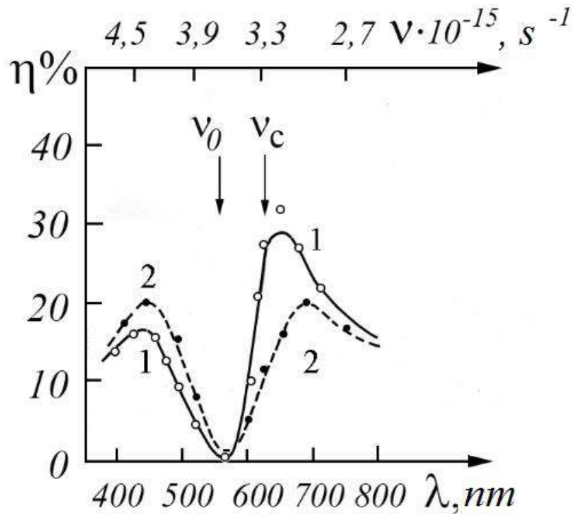
Fig.3.17. Spectral dependences DE lattice. Experimental values \eta : ● – for a symmetrical band \Delta D(\omega) ; ○ – for asymmetric band \Delta D(\omega) .
