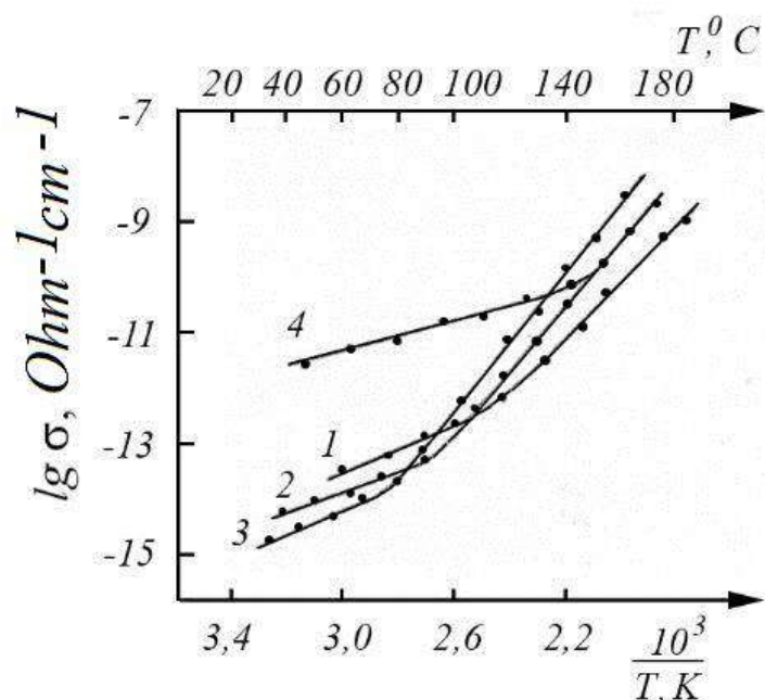
Fig.2.2. Temperature dependence of static (1–3) and dynamic conductivities at \omega=500 Hz (4) for samples with different sulfur content: 1 – As_2S_3 ; 2 – As_{25}S_{75} ; 3 – As_{20}S_{80} ; 4 – As_{25}S_{75} .
