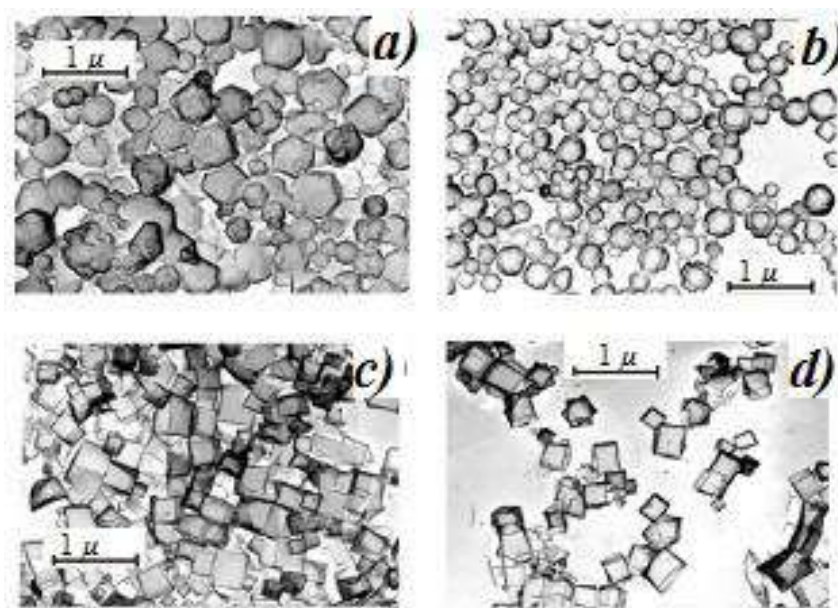
Fig.1.5. Photomicrographs of \text{CaF}_2 aqueous suspensions obtained with different pF : a) 1,0; b) 1,65; c) 2,0; d) 3,0.
