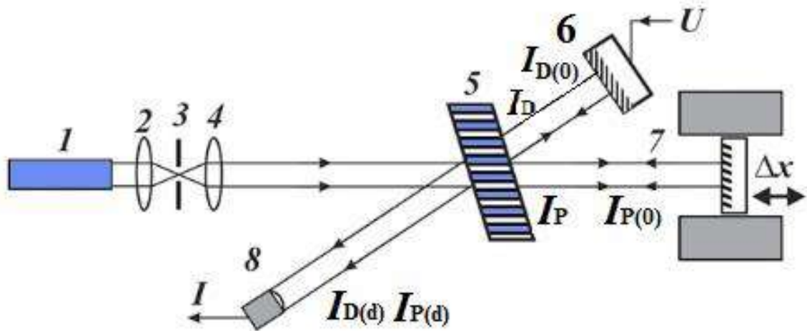
Fig.4.7. Schematic diagram of measuring linear displacements (non-contact method).
