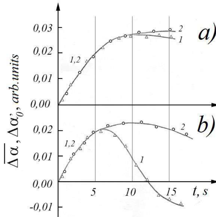
Fig.3.10. Kinetics of change \Delta\alpha'_0 (1) and \overline{\Delta\alpha} (2) when recording a three-dimensional lattice in \text{As}_2\text{S}_3 by He-Ne laser radiation for T ( ^{\circ}\text{C} ): a) -100 ; b) -150 . \Delta\alpha'_0 = \Delta\alpha_0 \cos \Delta\psi ; \Delta\alpha_0 > 0 , \cos \Delta\psi = \pm 1 .
