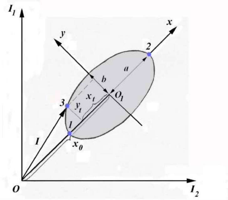
Fig.4.6. The trajectory described by the end of the vector I when the phase mismatch between the beams changes from 0 to 2\pi .
