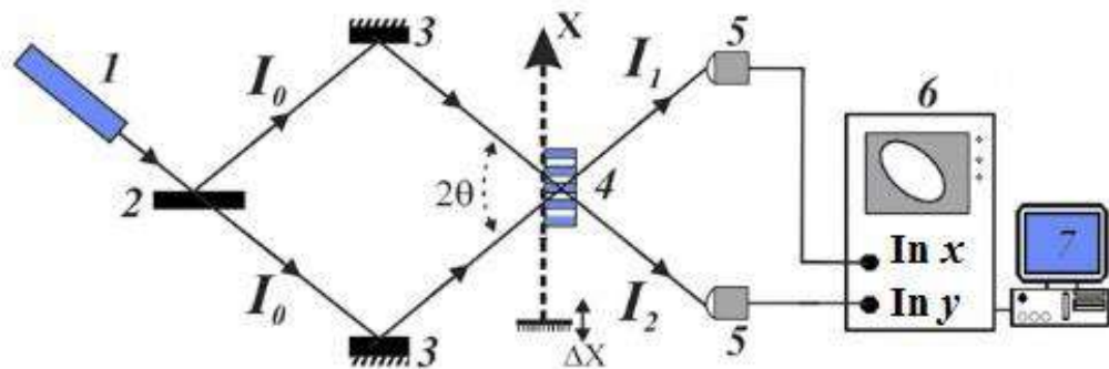
Fig.4.5. Schematic diagram of measuring linear displacements (contact method).
