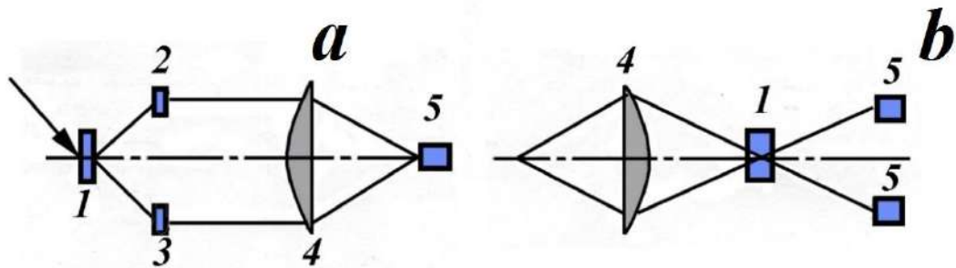
Fig.4.4. Scheme of use of three-dimensional passing diffraction gratings in transmitting ( a ) and receiving ( b ) paths of LDA. 1, 2, 3 – three-dimensional gratings, 4 – lenses, 5 – photodetectors.
