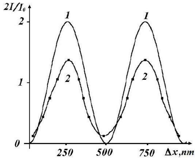
Fig.4.8. Dependence of the magnitude of the output signal I from the photodiode 8 (Fig.4.7) on the shift \Delta x of the object.
