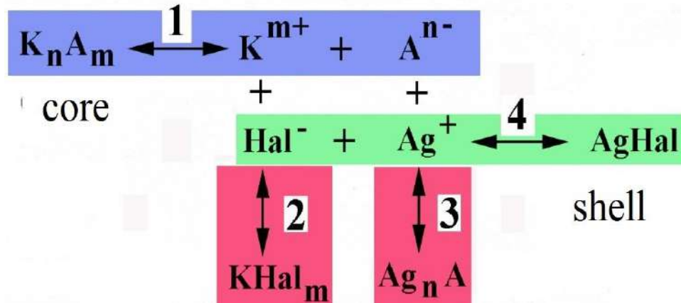
Fig.1.1. Scheme of chemical reactions when building a silver halide shell AgHal on a non-silver core K_n A_m .
