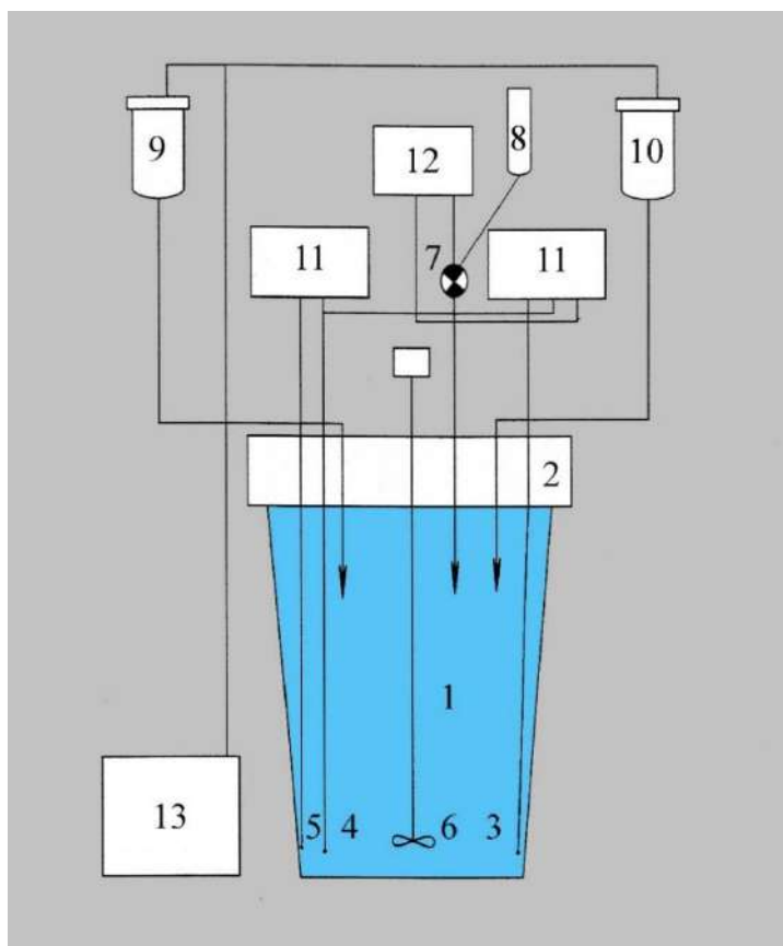
Fig.1.4. Principal scheme of the experimental installation for the synthesis of non-silver nuclei: 1 – thermostated reactor; 2 – cover; 3 – selective electrode; 4 – reference electrode; 5 – pH electrode; 6 – agitator with drive; 7 – solenoid valve automatic titration unit; 8, 9, 10 – vessels for solutions; 11 – ionometer EV-74; 12 – blocks of automatic titration BAT-15; 13 – compressor UK-16 M.
