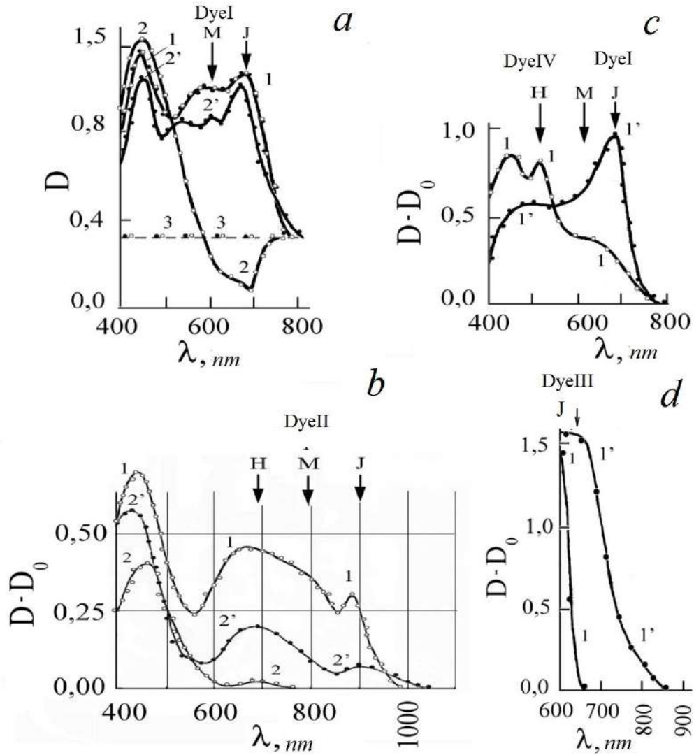
Fig.1.11. a ) Dependence of the optical density D of the exposed layers of emulsions of type B (1) and C (2,2') containing DyeI on the wavelength of the exposing light after development in the surface (1, 2) and deep (2') developers. The dashed line (3) indicates the optical density of the veil D 0 of unexposed emulsions of type B and type C and manifested in both surface and deep developers.
