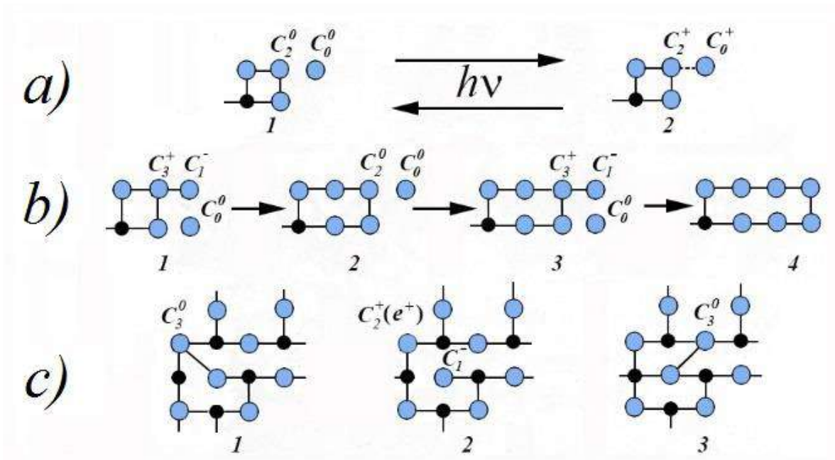
Fig.3.11. Creation of sulfur clusters as a result of diffusion of D^0 centers ( a and b ) in the compounds of the composition As-S with excess sulfur and the mechanism of diffusion D^0 centers in \text{As}_2\text{S}_3 compounds ( c ). The solid lines show the usual covalent bonds between arsenic ( \bullet ) and sulfur ( \circ ) atoms. The dotted line indicates the localized exciton.
