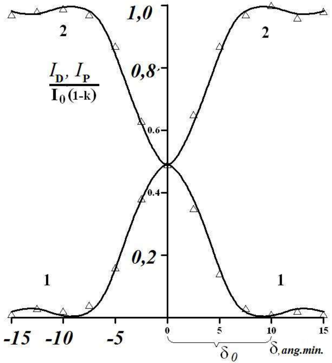
Fig.4.1. Angular dependence of light fluxes: 1 – diffracted I_D , 2 – passing I_P , from the change of the angle of incidence of the lattice of light flux I . Solid line – theoretically calculated by formulas (4.1) and (4.2), symbol \Delta – experimental values.
