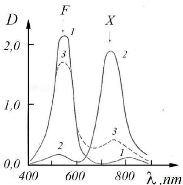
Fig.3.13. The absorption spectra of the KCl crystal before and after recording at T=270^{\circ}\text{C} (taken at room temperature).
