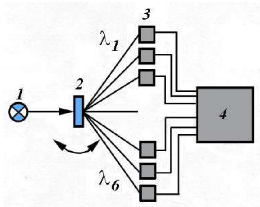
Fig.4.10. Schematic diagram of a multichannel spectroradiometer with HOE: 1 – light source, 2 – HOE, \lambda_i, i = 1, \dots, n – wavelengths of the emitted light flux, 3 – photodetectors, 4 – analyzer.
