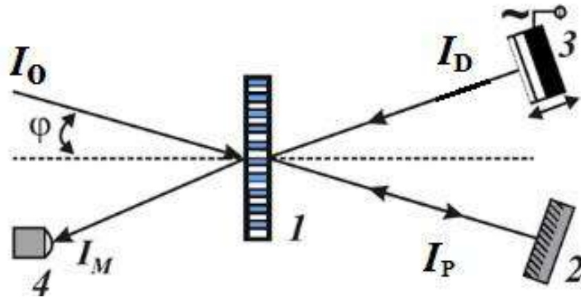
Fig.4.3. Two-beam scheme of optical radiation modulation: 1 – three-dimensional diffraction grating; 2 – a mirror; 3 – mirror on piezoceramics; 4 – photodetector.
