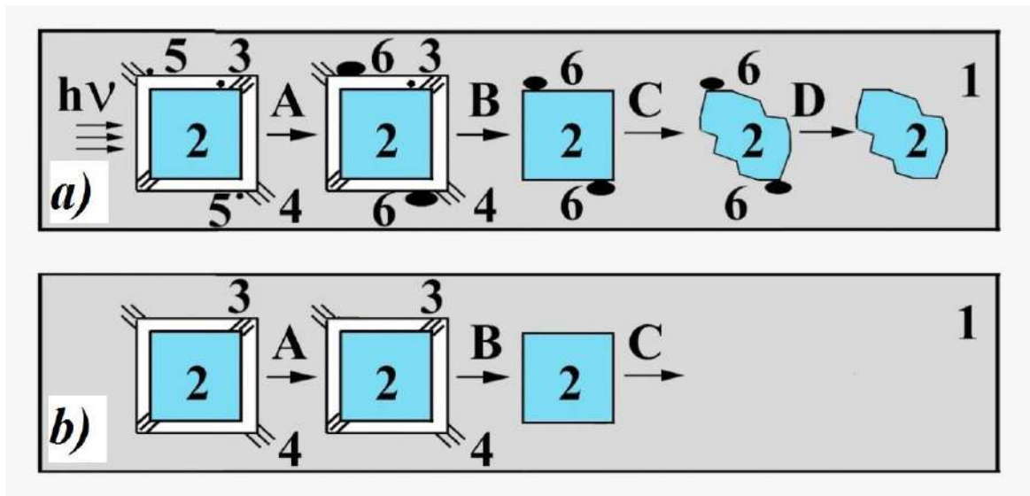
Fig.3.1. Processes occurring in illuminated (antinodes, row a ) and unilluminated (nodes, row b ) areas of the elementary hologram.
