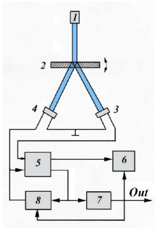
Fig.4.15. Schematic diagram of the angle of the measuring device: 1– emitter; 2 – HOE; 3, 4 – photodetectors; 5 – differential amplifier; 6 – display unit; 7 – three-stable comparator; 8 – gain regulator.
