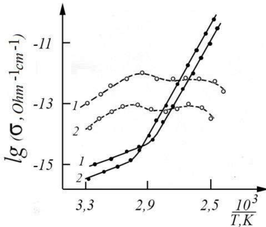
Fig.2.13. Dependence of conductivity (solid curve) and photoconductivity (dashed) on temperature for As_{20}S_{80} , measurement
