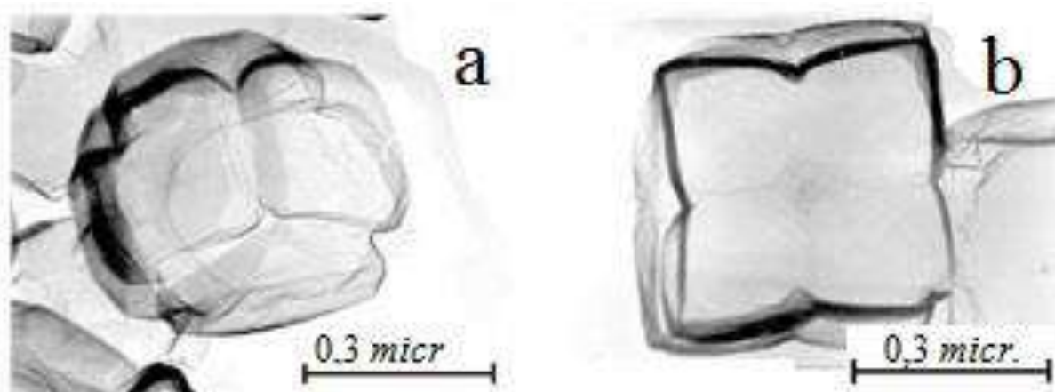
Fig.1.7. Photomicrographs of CaF_2 microcrystals precipitated at pF 1,65 (a) and 1,75 (b). Replicas with particles of the solid phase of the suspension are treated with a solution Al_2O_3 .
