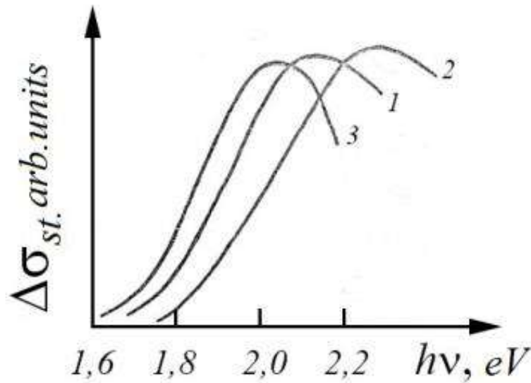
Fig.2.18. Spectral dependences of stationary photoconductivity for unexposed sample (curve 1) and the same sample exposed in the modes described above (curve 2 – irradiated with He-Ne laser at 160°C, curve 3 – irradiated with xenon lamp light at 20°C).
