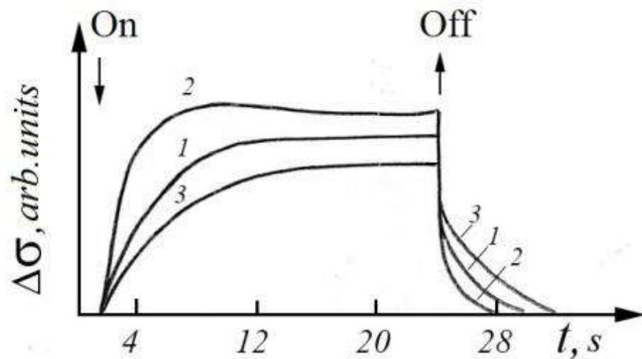
Fig.2.16. Kinetics of photocurrent for \text{As}_2\text{S}_3 at T=55^\circ\text{C} and \omega = 290 \text{ Hz} : 1 – sample annealed at 180^\circ\text{C} for 15 min; 2 – exposed to He-Ne laser radiation at 160^\circ\text{C} for 15 min ( I=0,15 \text{ W/cm}^2 ); 3 – exposed to xenon lamp radiation at 20^\circ\text{C} for 7 hours (lamp power \sim 500 \text{ W} ).
