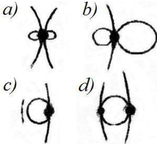
Fig.3.24. Scattering patterns for a hologram written in blue laser ( \lambda=488\text{ nm} ) and read in red ( \lambda=633\text{ nm} ).
