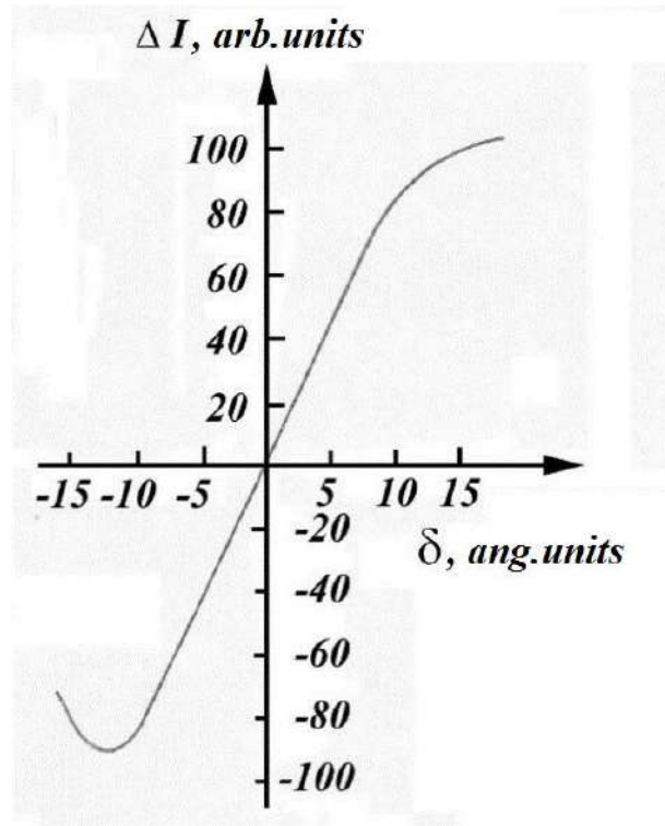
Fig.4.12. Angular dependence \Delta I = I_P - I_D . (Angular dependences I_P and I_D are shown in Fig.4.11).
