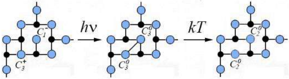
Fig.2.21. "Healing" of its own defects in the material under the action of light, which leads to the creation of normally coordinated atoms (● – sulfur, ● – arsenic).
