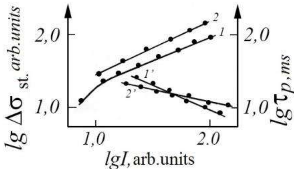
Fig.2.15. Dependence \Delta\sigma_{st} (curves 1, 2) and \tau_p (curves 1', 2') on the intensity of exciting light: 1, 1'– the sample is annealed at 180°C for
