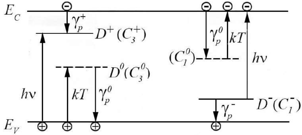
Fig.2.7. Energy levels in the band gap of CGS and the scheme of optical ( h\nu ), thermal ( kT ) and recombination ( \gamma_p ) transitions. The direction of the arrows indicates the movement of electrons.
