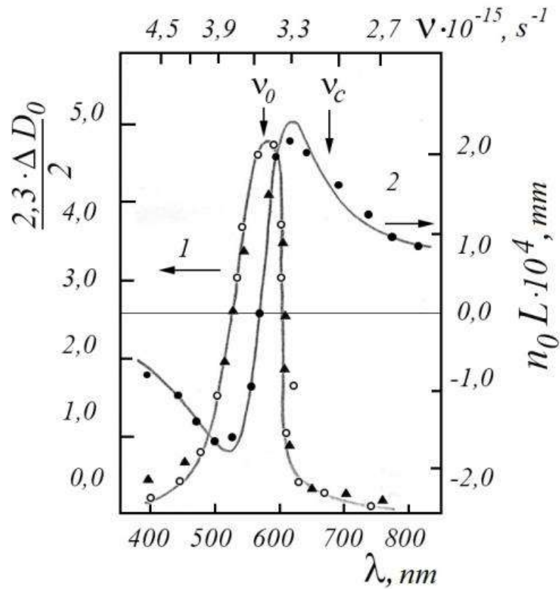
Fig.3.15. Dispersion \Delta D_0 , \Delta n and \bar{D} lattice (NaCl crystal).
