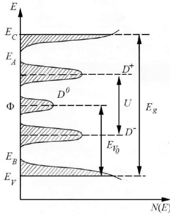
Fig.2.1. Energy spectra of CGS. Localized states are hatched. \Phi – Fermi level.
