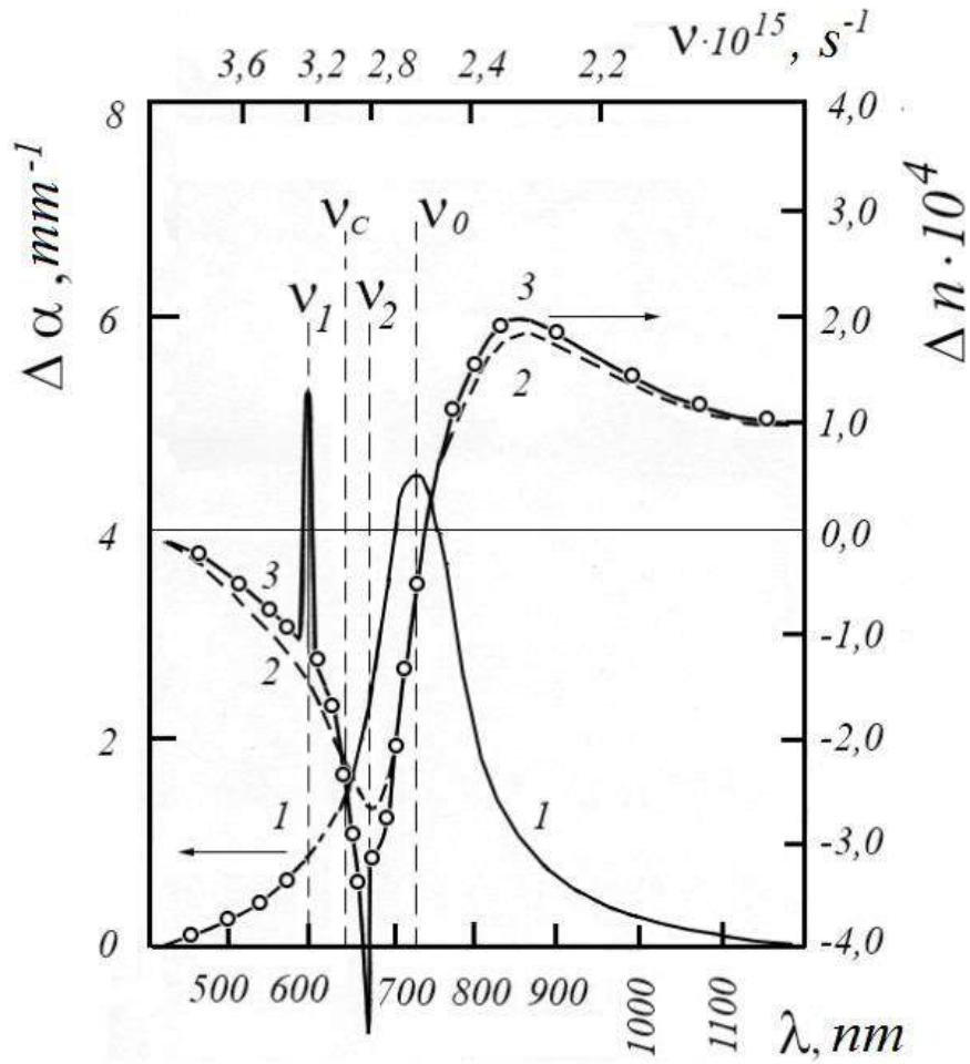
Fig.3.19. Spectral dependences \Delta n(\lambda) in the case of selective destruction of colloidal centers in KCl :
