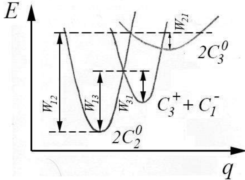
Fig.2.22. Configuration-coordinate diagram of photostructural transformations in system materials As-S.
