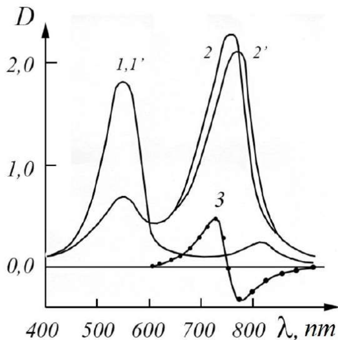
Fig.3.20. The absorption spectra of the KCl crystal before (1, 1') and after (2, 2') the recording of the holographic lattice. 1, 2 and 1', 2' are measured, respectively, by linearly polarized light, the electric vector of which is parallel and perpendicular to the electric vector of the recording beam; 3 – dichroism curve (difference of curves 2 and 2').
