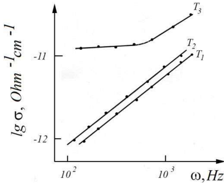
Fig.2.3. Frequency dependence of conductivity As_2S_3 : T_1=55^\circ C ; T_2=90^\circ C ; T_3=140^\circ C .
