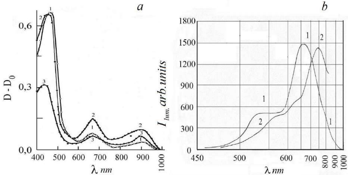
Fig.1.15. a ) Optical dependence densities D - D_0 from the wavelength of light exposing layers of emulsions of type F with DyeI after development in the surface (1) and deep (2, 3) developers with oxidation of surface centers t (min): 2 – 1; 3 – 20,
