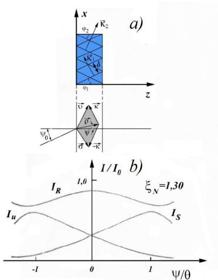
Fig.4.14. a) Vector diagram explaining the diffraction of light on a three-dimensional combined grating; b) the dependence of the intensities of the transmitted beam I_R and diffracted beams I_s and I_u from the angle of incidence of light \psi , which is normalized to the angle of Bragg \theta .
