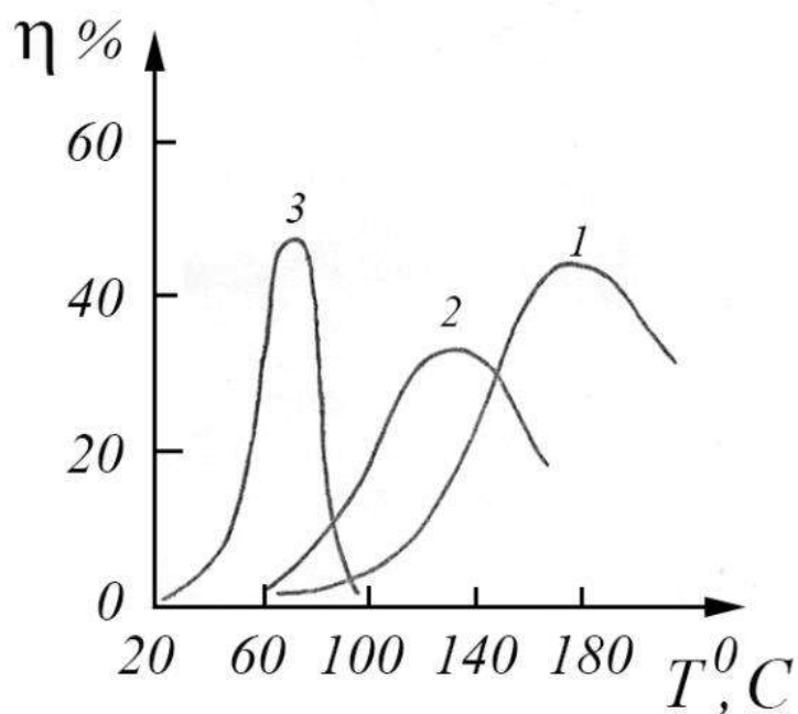
Fig.3.9. Dependence DE elementary gratings recorded at the same absorption energy, from the heating temperature of the plates As_2S_3 (1) and As_{25}S_{75} (2, 3); 2 – before thermal annealing; 3 – after thermal annealing at T \approx 150^\circ C for 15 minutes.
