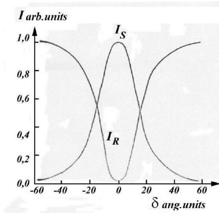
Fig.4.11. Angular dependences I_P and I_D for lattices with DE \eta = 100\% .
