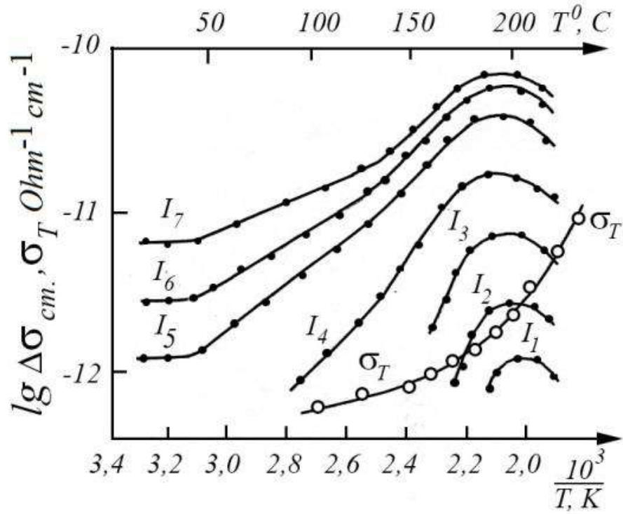
Fig.2.9. Temperature dependence of dark ( \Delta\sigma_T ) and stationary ( \Delta\sigma_{st} ) photoconductivity As_2S_3 ( \omega=290 Hz), which was measured at different intensities of exciting light ( I_4 < I_5 < I_6 < I_7 ).
