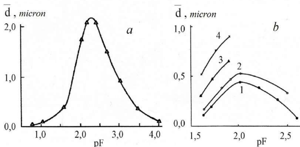
Fig.1.6. Dependence of the average size of \text{CaF}_2 microcrystals on pF :
