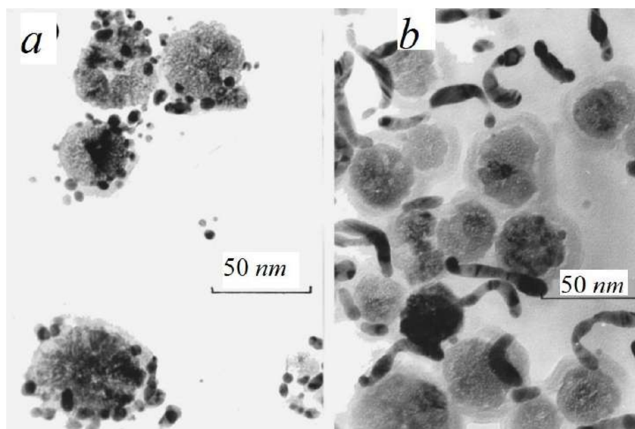
Fig.3.2. Microphotographs of developed microcrystals, especially fine-grained emulsions: a ) – heterophase composite system; b ) – obtained by mechanical mixing, especially fine-grained suspensions AgHal and CaF_2 .
