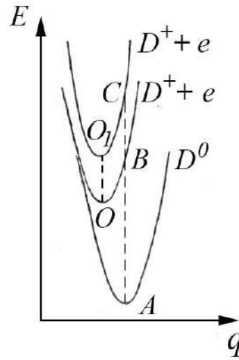
Fig.2.23. Level-zone optical transitions with the participation of a center with strong electron-phonon interaction.
