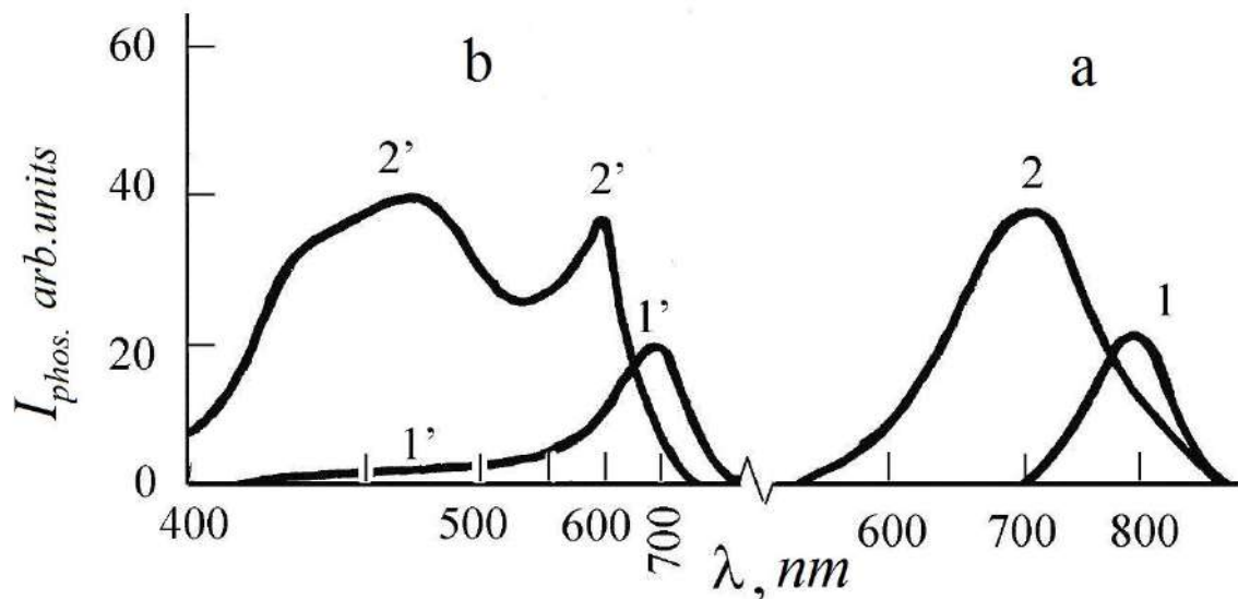
Fig.1.13. The spectra ( T=77K ) of phosphorescence (a) and phosphorescence excitation (b) of emulsions ( \bar{d}\approx 0,05 \mu m ) contain DyeI: 1, 1'– type A; 2, 2'– type B:
