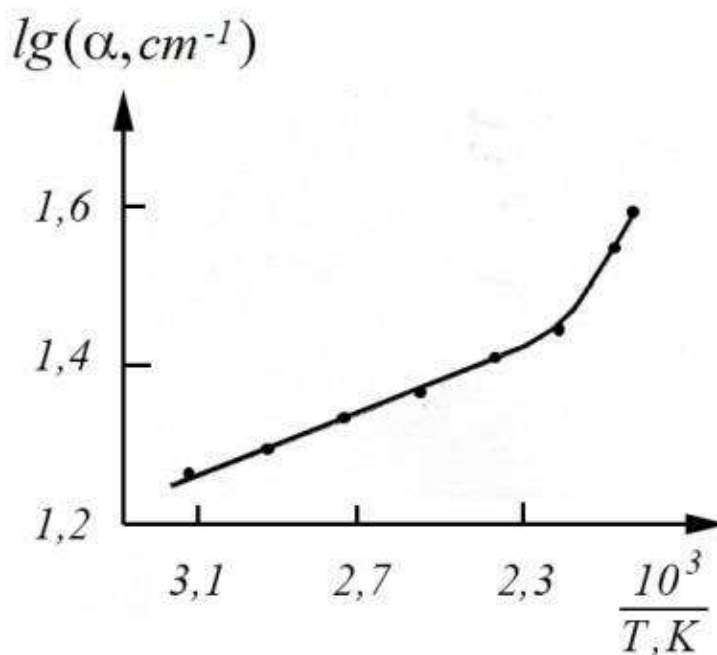
Fig.2.6. Temperature dependence of the absorption coefficient on the wavelength of He-Ne laser radiation ( \lambda = 632,8 \text{ nm} ). The energy of the linear section is \approx 0,03 \text{ eV} .
