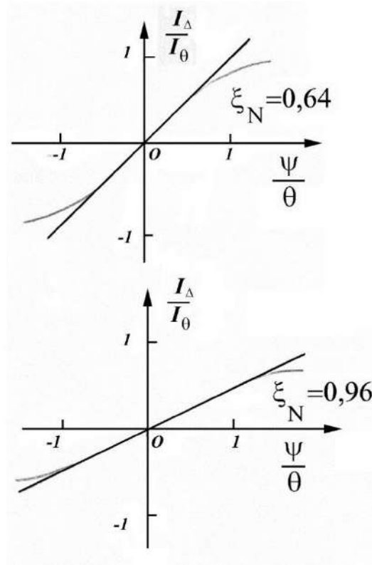
Fig.4.17. Dependence I_{\Delta} = I_s - I_u on the angle of incidence \psi light normalized to the Bragg angle \theta on HOE at various parameters \xi_N .
