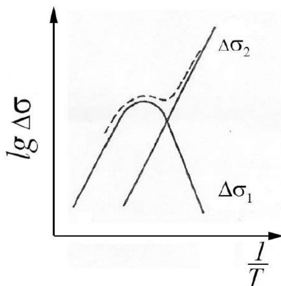
Fig.2.14. Temperature dependence of photoconductivity on localized (hopping \Delta\sigma_1 ) and nonlocalized (band \Delta\sigma_2 ) states. Dotted curve – the resulting dependence of photoconductivity on temperature.
