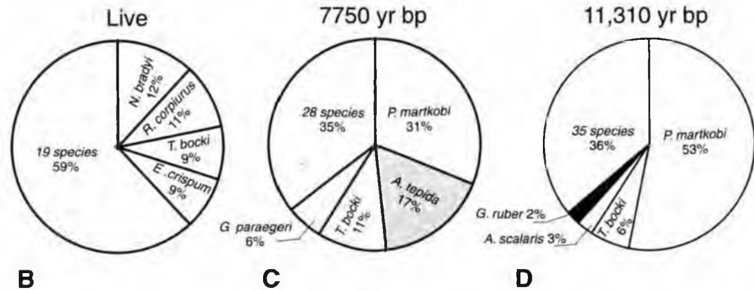
Figure 7. Core 80b: The dotted line indicates the Holocene-Pleistocene boundary. (A) distribution of grain size, P/B, RDS, A. tepida , CaCO 3 and C org in the sedimentological column; (B–D) diagrams showing dominant and accessory foraminiferal species in the (B) live (Rose Bengal stained) assemblage; (C) core-top Holocene (7750 yr bp) assemblage; (D) late Pleistocene (11,310 yr bp) assemblage.
