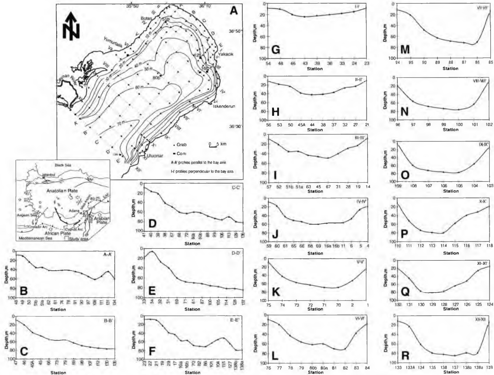
Figure 1. (A) Map of Iskenderun Bay showing the location of the study area, the bathymetry in meters, sampling profiles, and the grab (labeled black dots) and core (labeled black squares) locations. BZS—Bitlis-Zagros suture; DSFZ—Dead Sea fault zone; EAF—Eastern Anatolian fault; NAF—North Anatolian fault. (B–F) Cross-sections of the bottom obtained parallel to the shore showing the bottom morphology. Figure (G–R) Cross-sections of the bottom obtained perpendicular to the shore.
