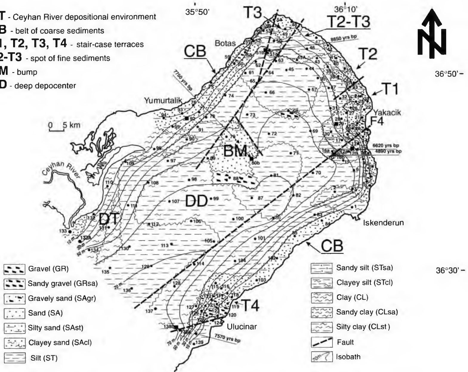
Figure 2. Lithological map of Iskenderun Bay showing the bathymetrical distribution of lithotypes, stair-case tectonic structures, and faults.
