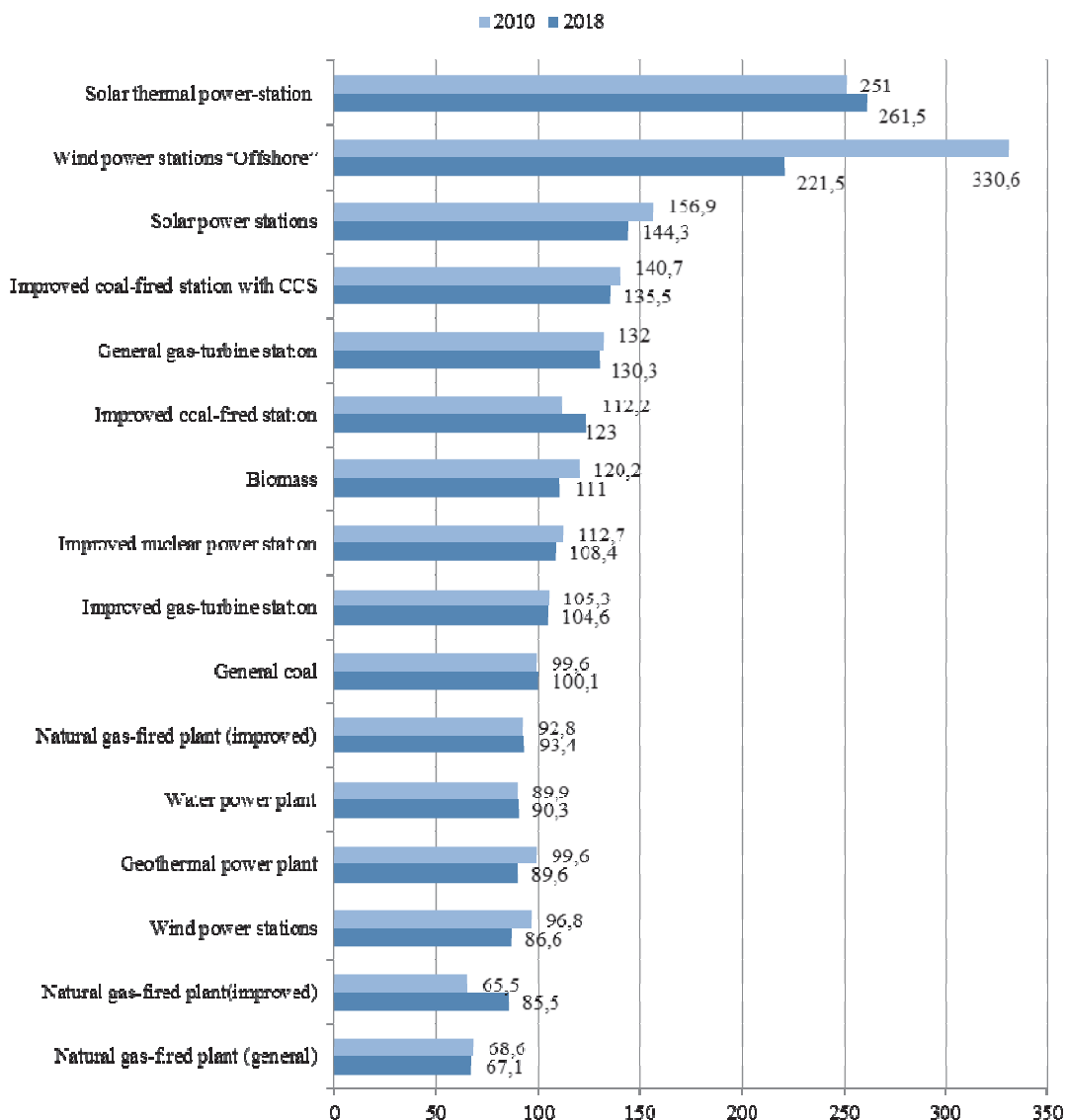
Figure 1. Evaluation of the average fixed cost price of electricity of power stations in 2010 and power stations being put into operation in 2018, $/MWh.
