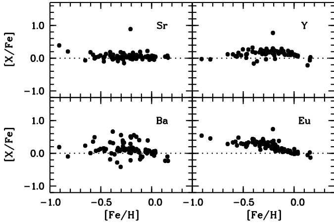
Fig. 9. Heavy elements vs. [Fe/H] for the sample stars.
