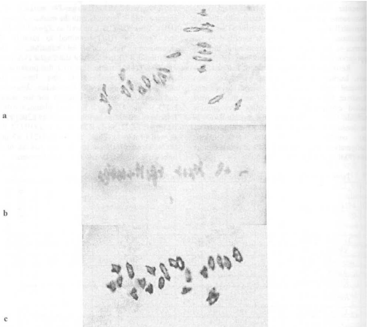
Fig. 1. The highest chromosome associations at meiotic MI of F 1 hybrids between cv. Od267 and (a) line E242_97-1: 20^{11c} + 1^{11o} ; (b) line H274_97: 19^{11c} + 1^{11o} + 2^1 ; (c) line E217_97 (plants without 1B_L|1R_S translocation): 21^{11c} (590 \times )
