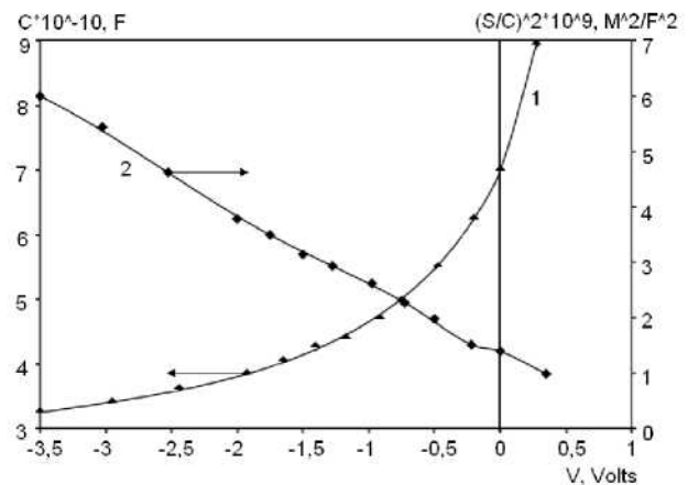
Fig. 2. Capacitance-voltage characteristics of Cr-ZnSe contact.
