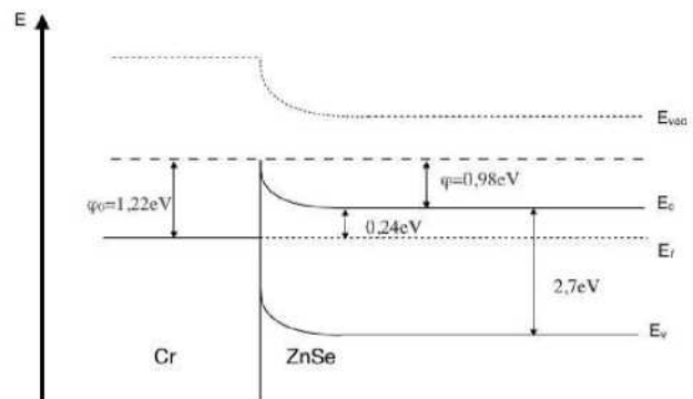
Fig. 3. Energy diagram of the Cr-ZnSe contact balance.
