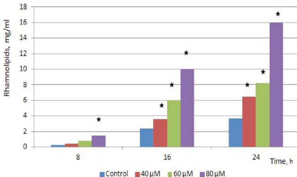
Fig. Kinetics of P. aeruginosa ONU 301 rhamnolipids biosynthesis in presence of quinolone signal molecule
