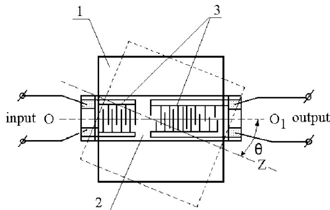
Fig. 3. The NCC scheme . 1 — piezoelectric soundconductor, 2 — dielectric plate with IDC, 3 — IDC
