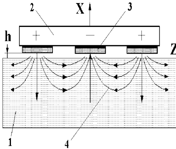
Fig. 5. Geometry SAW noncontact excitation task. piezoelectric half-space, 2 — dielectric plate, 3 — IDC electrodes, 4 — electromagnetic field lines of force.
