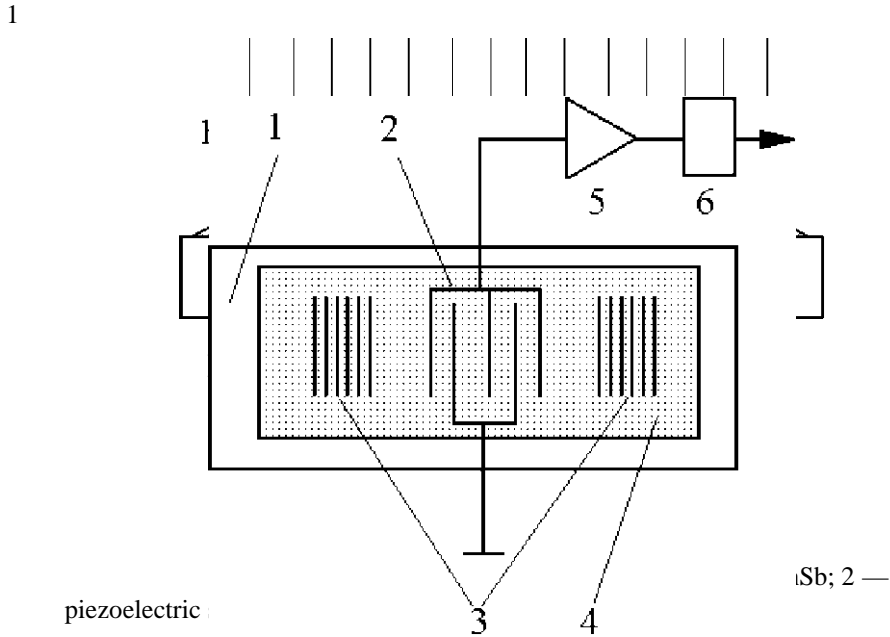
Fig. 7. Acoustoelectronic IR- radiation sensor. 1 — piezoelectric soundconductor (LiNbO3); 2,3 — SAW resonator structure; 4 — InSb film; 5 — amplifier; 6 — LFF.
