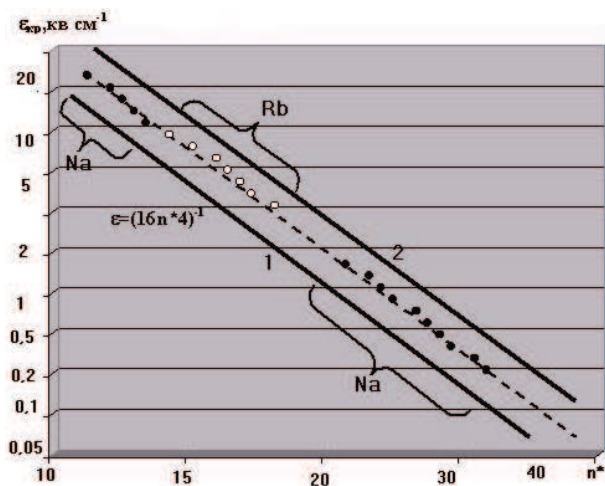
Fig.1. Critical electric field strength in dependence upon effective quantum number n^* for atoms of Na, Rb: dots – experiment (see [1]); solid line 1 – theoretical estimate on the basis of classical model; solid line 2 – calculation within the H-like approximation; dotted line –our data (eq.(1))
