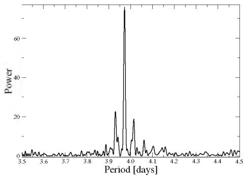
Figure 6: Fourier power spectrum of the Polaris Aa RV measurements for the 2015 – 2020 data.
